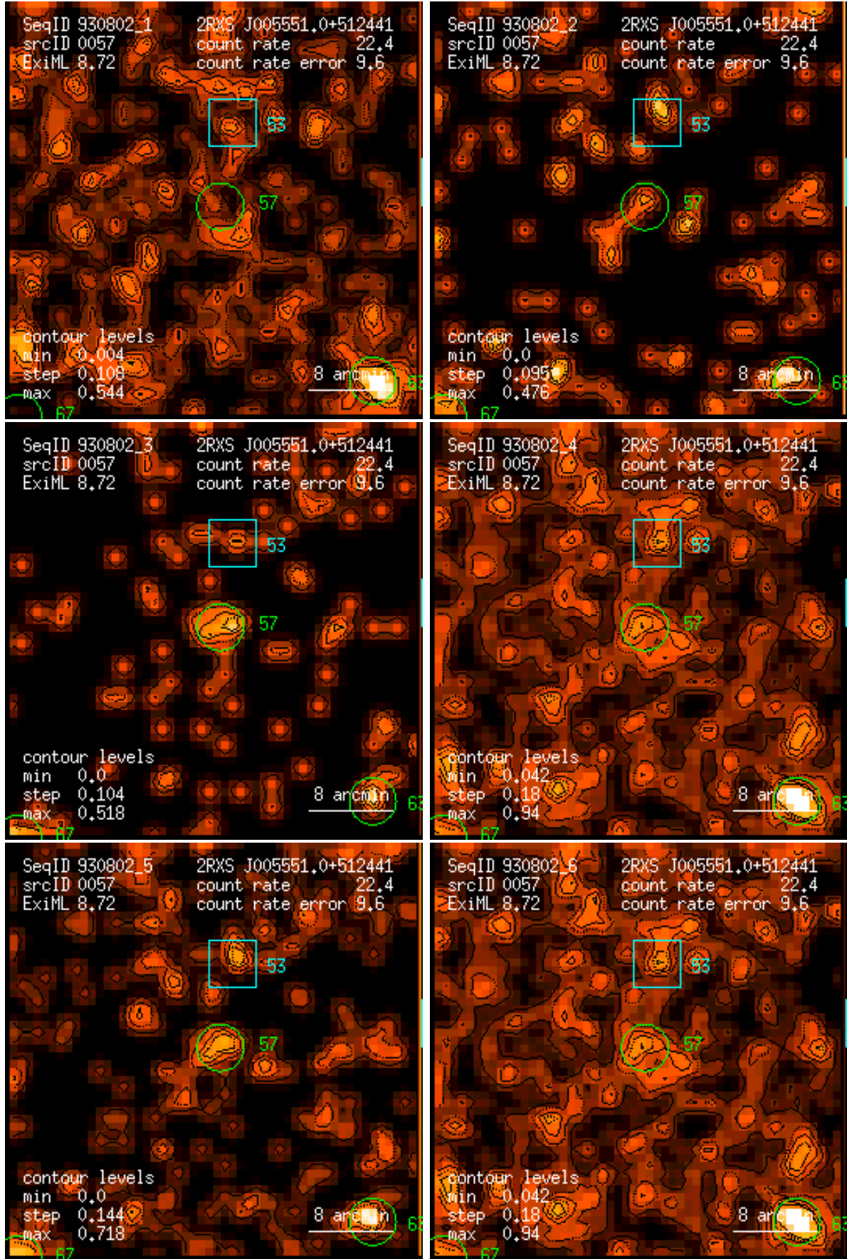
Figure 57: RASS 930802: detection 0057: band rate images, Gaussian filter: (1) PSPC channels 11 – 41, (2) 52 – 90, (3) 91 – 201, (4) 11 – 235, (5) 52 – 201, (6) 11 – 201. Broad band rates in counts/ks. Band rate contour levels in counts/ks/arcmin 2 .
