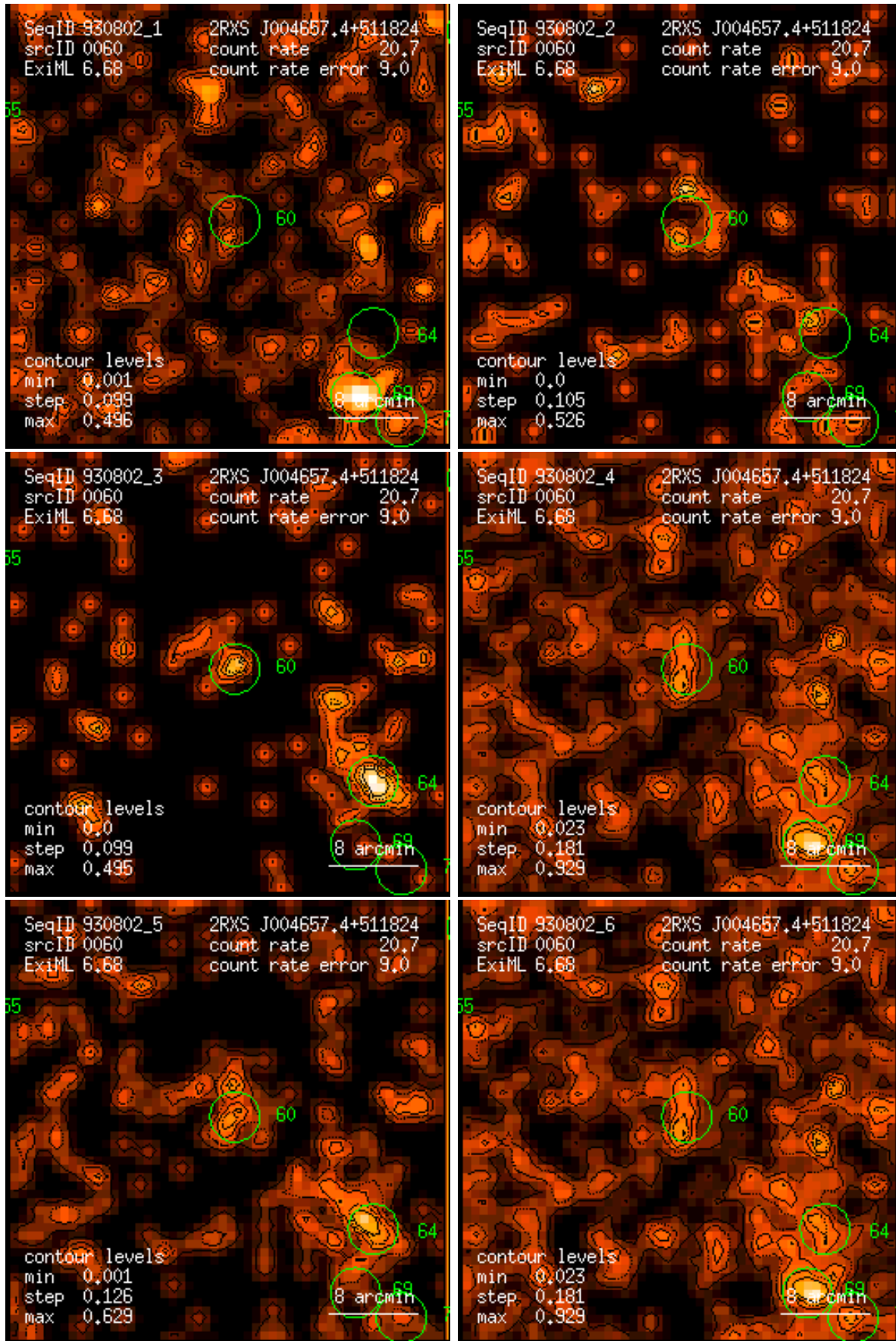
Figure 60: RASS 930802: detection 0060: band rate images, Gaussian filter: (1) PSPC channels 11 – 41, (2) 52 – 90, (3) 91 – 201, (4) 11 – 235, (5) 52 – 201, (6) 11 – 201. Broad band rates in counts/ks. Band rate contour levels in counts/ks/arcmin 2 .
