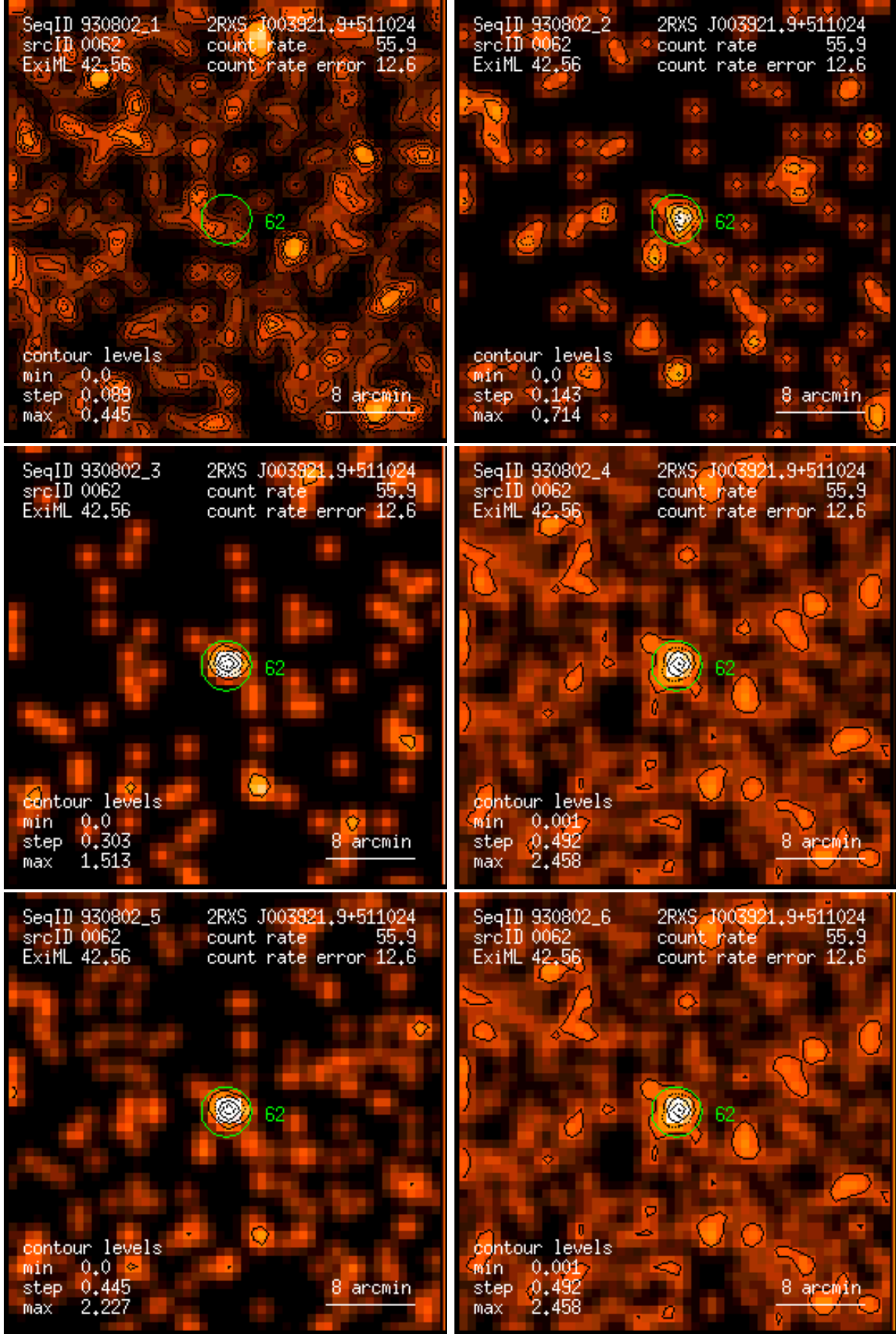
Figure 62: RASS 930802: detection 0062: band rate images, Gaussian filter: (1) PSPC channels 11 – 41, (2) 52 – 90, (3) 91 – 201, (4) 11 – 235, (5) 52 – 201, (6) 11 – 201. Broad band rates in counts/ks. Band rate contour levels in counts/ks/arcmin 2 .
