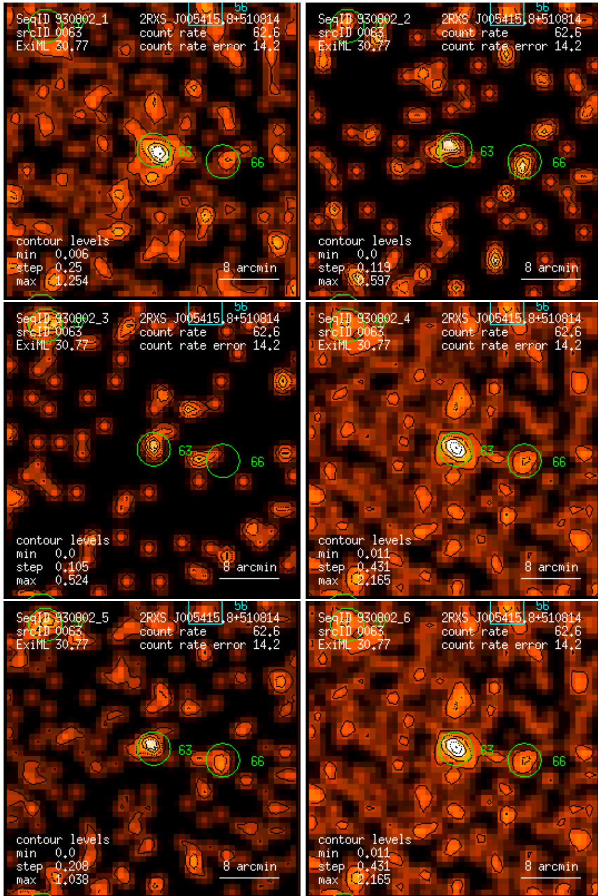
Figure 63: RASS 930802: detection 0063: band rate images, Gaussian filter: (1) PSPC channels 11 – 41, (2) 52 – 90, (3) 91 – 201, (4) 11 – 235, (5) 52 – 201, (6) 11 – 201. Broad band rates in counts/ks. Band rate contour levels in counts/ks/arcmin 2 .
