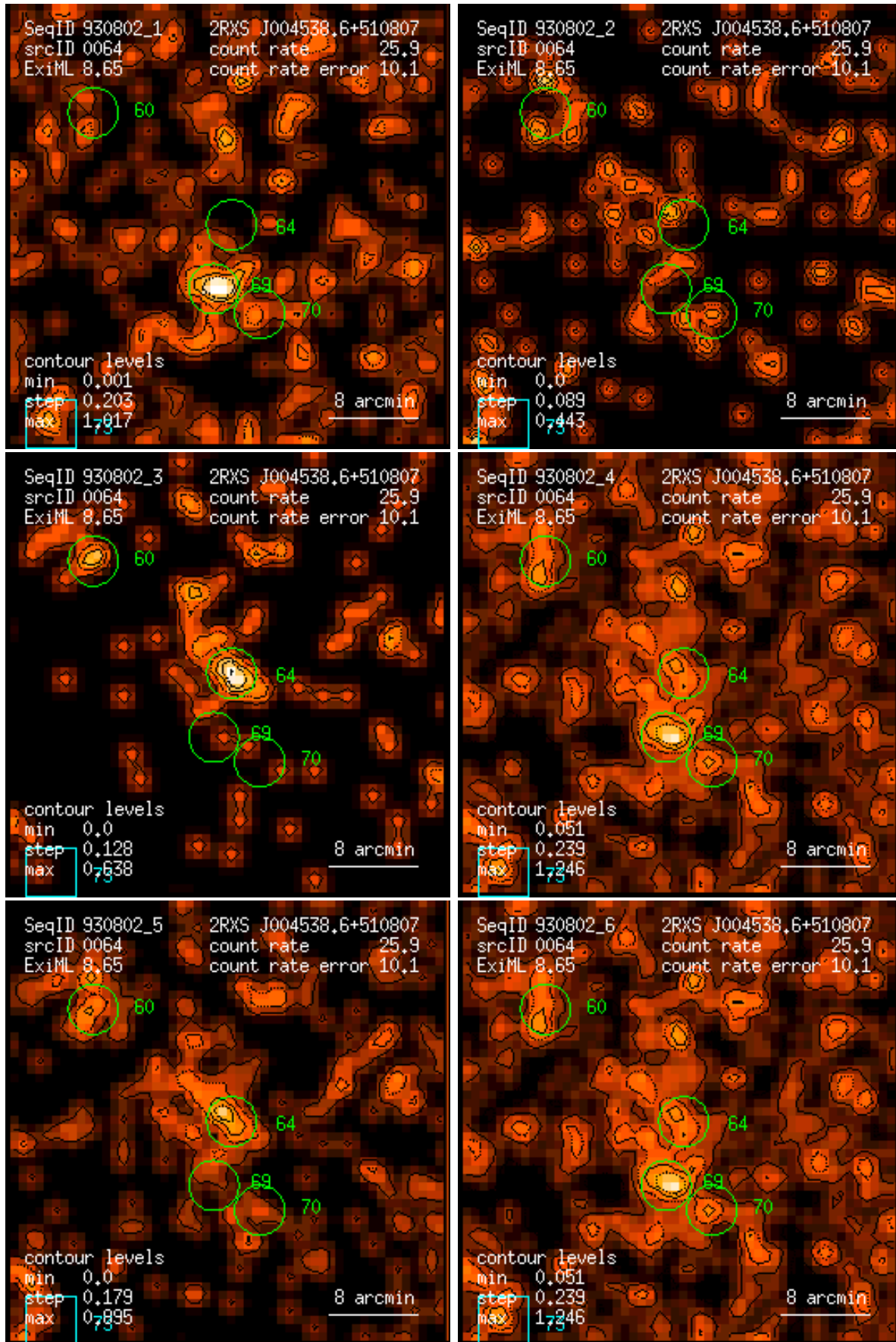
Figure 64: RASS 930802: detection 0064: band rate images, Gaussian filter: (1) PSPC channels 11 – 41, (2) 52 – 90, (3) 91 – 201, (4) 11 – 235, (5) 52 – 201, (6) 11 – 201. Broad band rates in counts/ks. Band rate contour levels in counts/ks/arcmin 2 .
