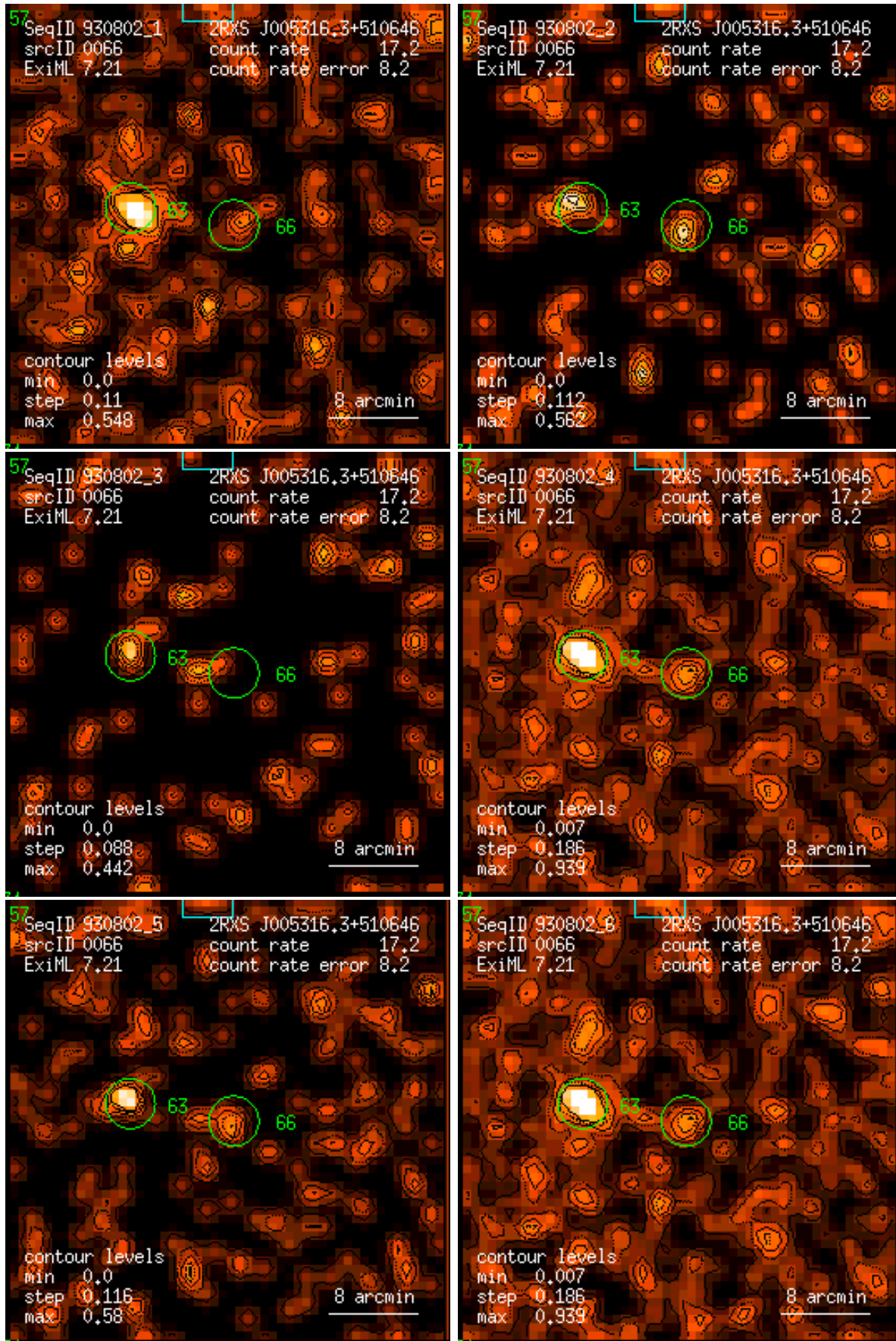
Figure 66: RASS 930802: detection 0066: band rate images, Gaussian filter: (1) PSPC channels 11 – 41, (2) 52 – 90, (3) 91 – 201, (4) 11 – 235, (5) 52 – 201, (6) 11 – 201. Broad band rates in counts/ks. Band rate contour levels in counts/ks/arcmin 2 .
