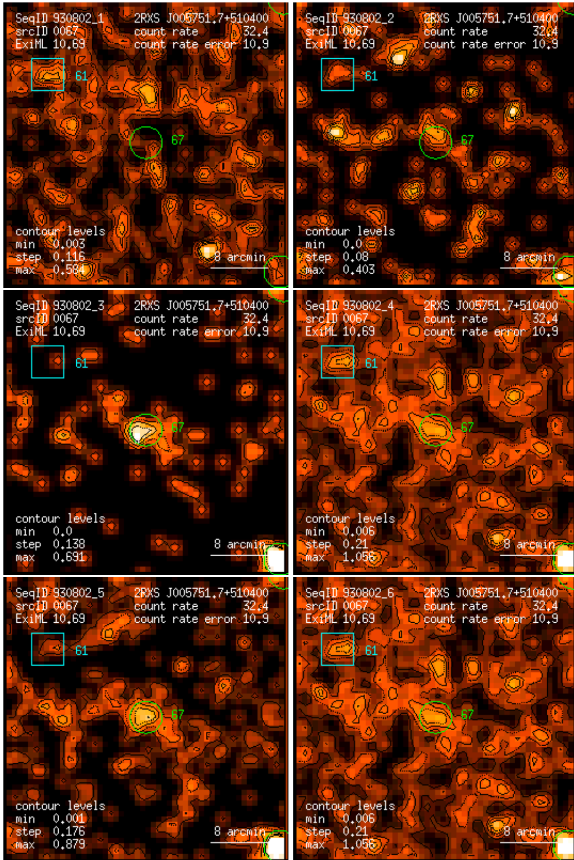
Figure 67: RASS 930802: detection 0067: band rate images, Gaussian filter: (1) PSPC channels 11 – 41, (2) 52 – 90, (3) 91 – 201, (4) 11 – 235, (5) 52 – 201, (6) 11 – 201. Broad band rates in counts/ks. Band rate contour levels in counts/ks/arcmin 2 .
