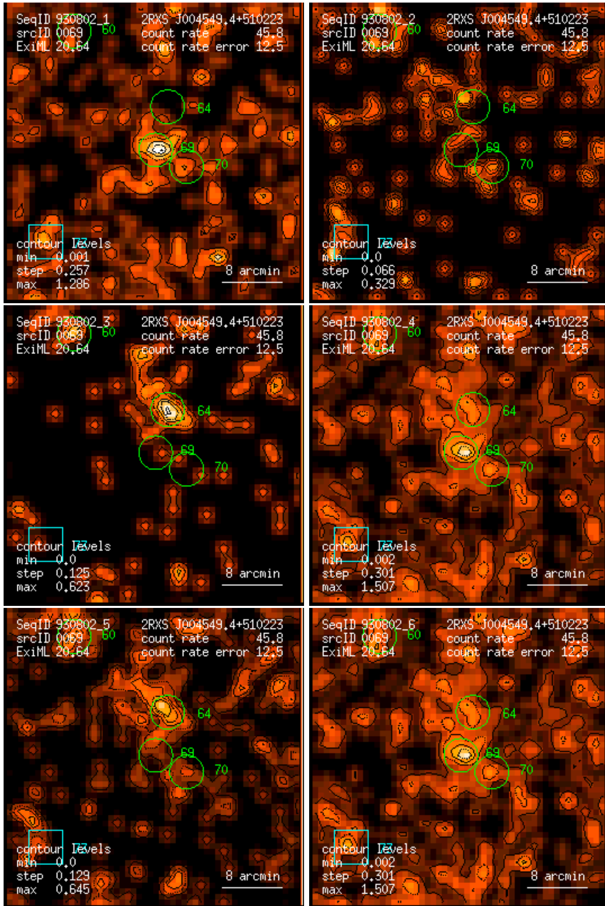
Figure 69: RASS 930802: detection 0069: band rate images, Gaussian filter: (1) PSPC channels 11 – 41, (2) 52 – 90, (3) 91 – 201, (4) 11 – 235, (5) 52 – 201, (6) 11 – 201. Broad band rates in counts/ks. Band rate contour levels in counts/ks/arcmin 2 .
