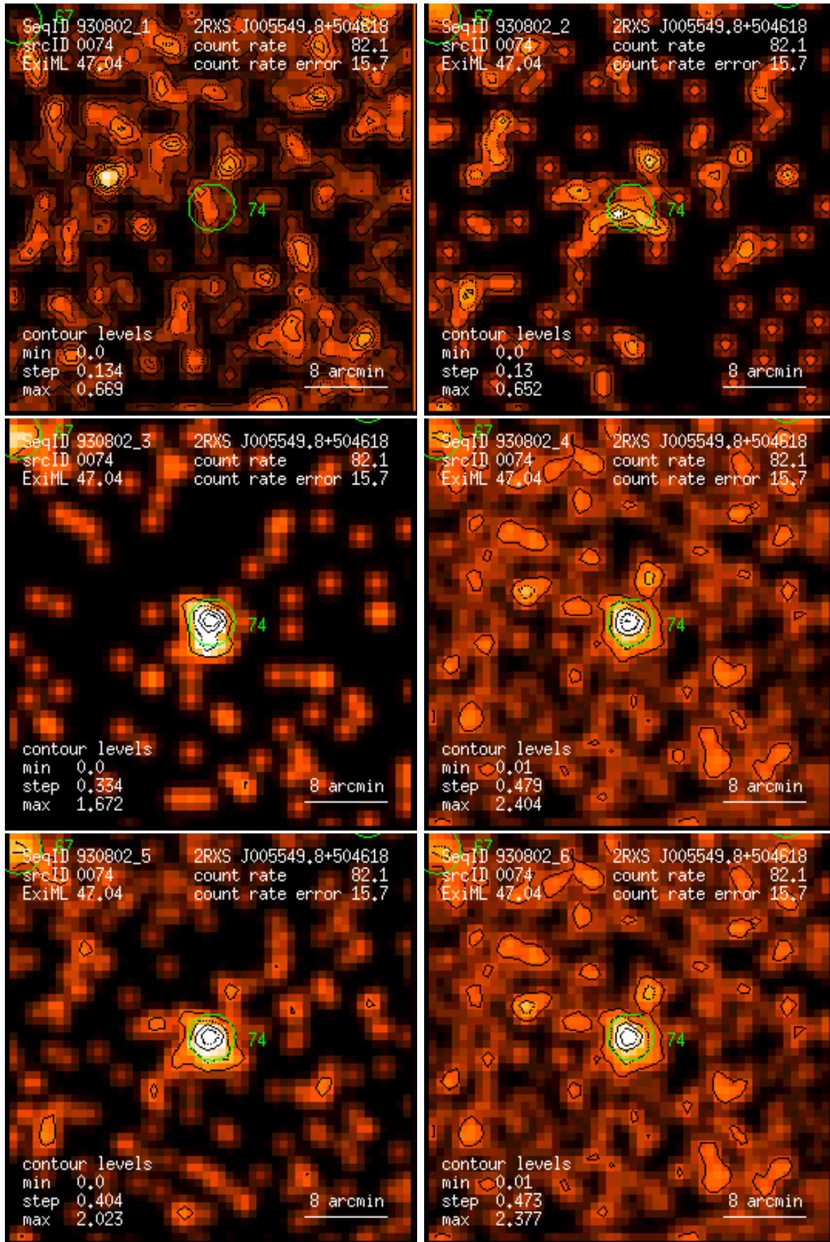
Figure 74: RASS 930802: detection 0074: band rate images, Gaussian filter: (1) PSPC channels 11 – 41, (2) 52 – 90, (3) 91 – 201, (4) 11 – 235, (5) 52 – 201, (6) 11 – 201. Broad band rates in counts/ks. Band rate contour levels in counts/ks/arcmin 2 .
