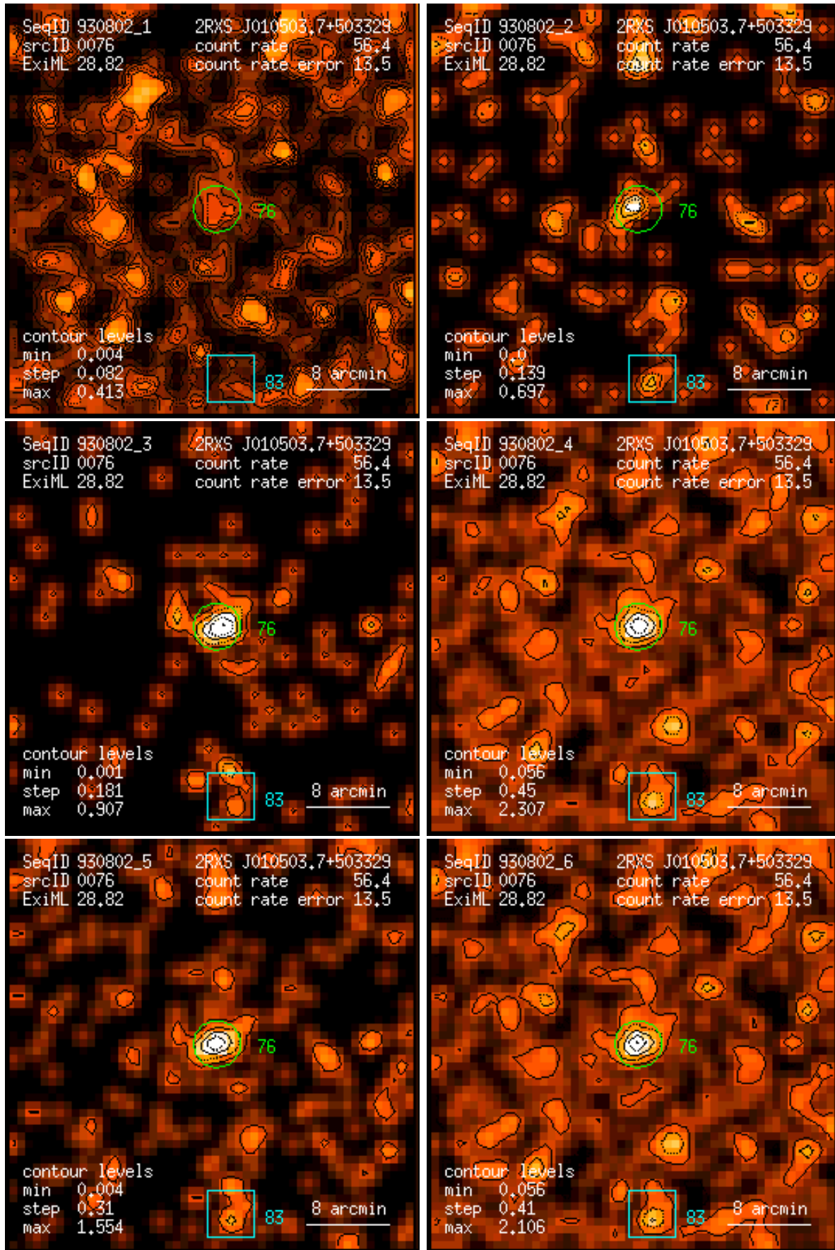
Figure 76: RASS 930802: detection 0076: band rate images, Gaussian filter: (1) PSPC channels 11 – 41, (2) 52 – 90, (3) 91 – 201, (4) 11 – 235, (5) 52 – 201, (6) 11 – 201. Broad band rates in counts/ks. Band rate contour levels in counts/ks/arcmin 2 .
