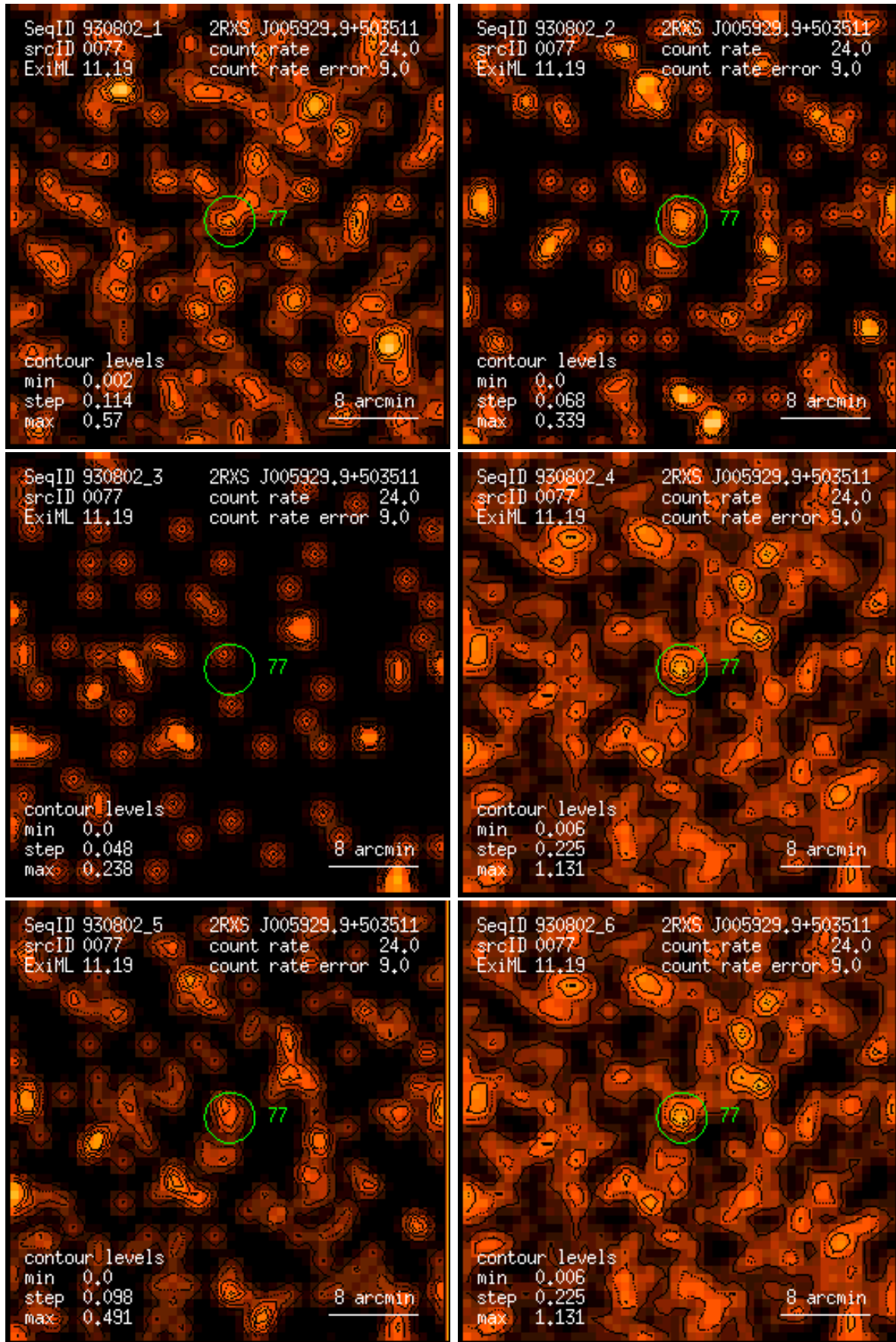
Figure 77: RASS 930802: detection 0077: band rate images, Gaussian filter: (1) PSPC channels 11 – 41, (2) 52 – 90, (3) 91 – 201, (4) 11 – 235, (5) 52 – 201, (6) 11 – 201. Broad band rates in counts/ks. Band rate contour levels in counts/ks/arcmin 2 .
