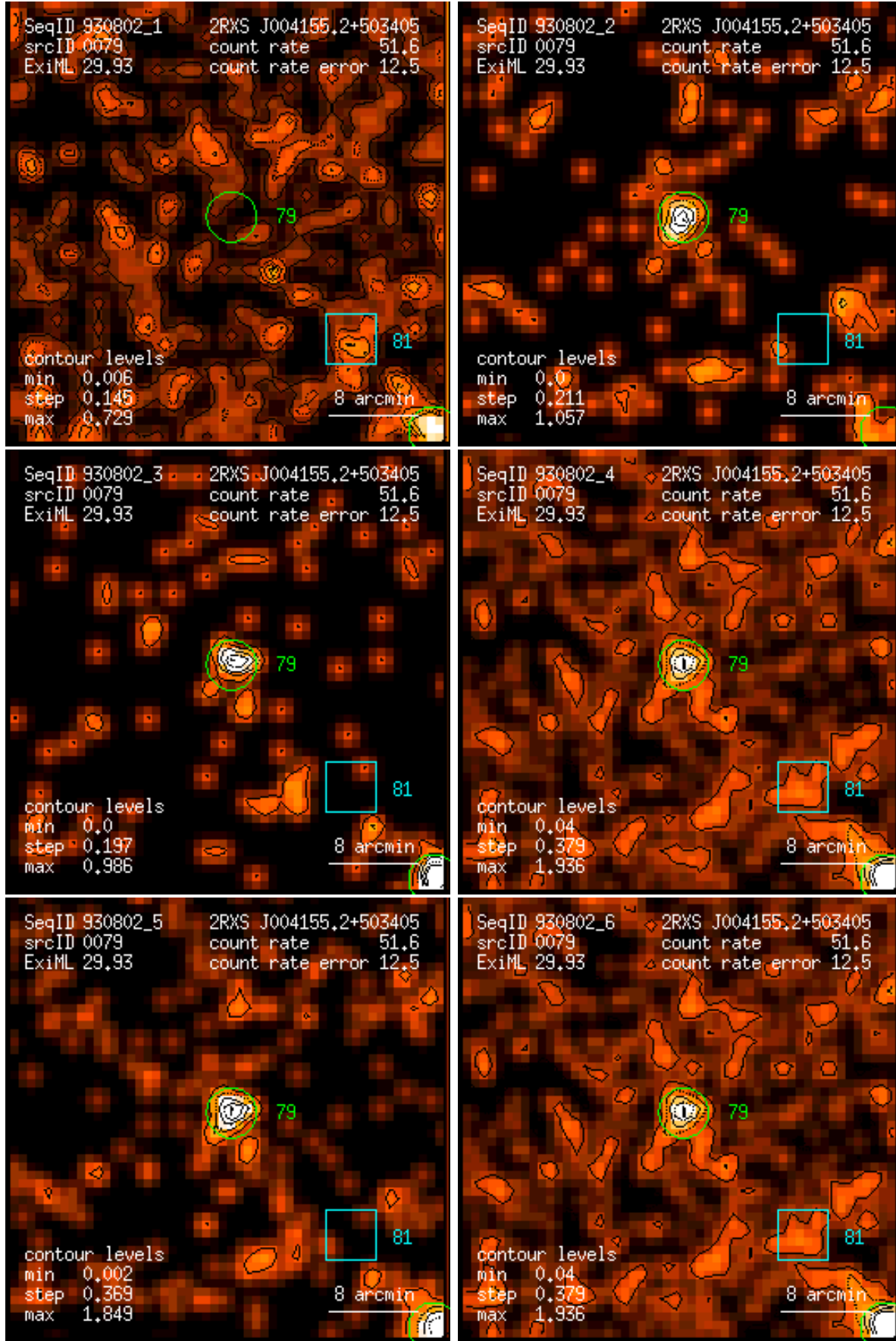
Figure 79: RASS 930802: detection 0079: band rate images, Gaussian filter: (1) PSPC channels 11 – 41, (2) 52 – 90, (3) 91 – 201, (4) 11 – 235, (5) 52 – 201, (6) 11 – 201. Broad band rates in counts/ks. Band rate contour levels in counts/ks/arcmin 2 .
