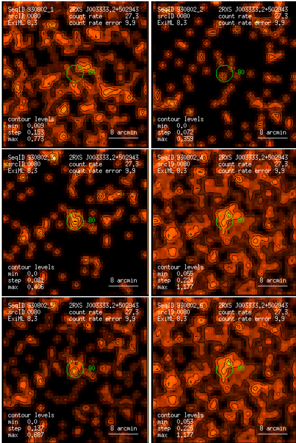
Figure 80: RASS 930802: detection 0080: band rate images, Gaussian filter: (1) PSPC channels 11 – 41, (2) 52 – 90, (3) 91 – 201, (4) 11 – 235, (5) 52 – 201, (6) 11 – 201. Broad band rates in counts/ks. Band rate contour levels in counts/ks/arcmin 2 .
