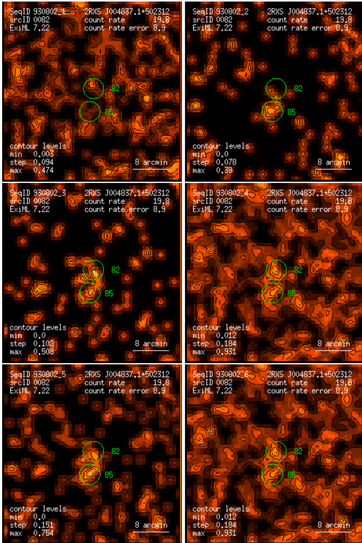
Figure 82: RASS 930802: detection 0082: band rate images, Gaussian filter: (1) PSPC channels 11 – 41, (2) 52 – 90, (3) 91 – 201, (4) 11 – 235, (5) 52 – 201, (6) 11 – 201. Broad band rates in counts/ks. Band rate contour levels in counts/ks/arcmin 2 .
