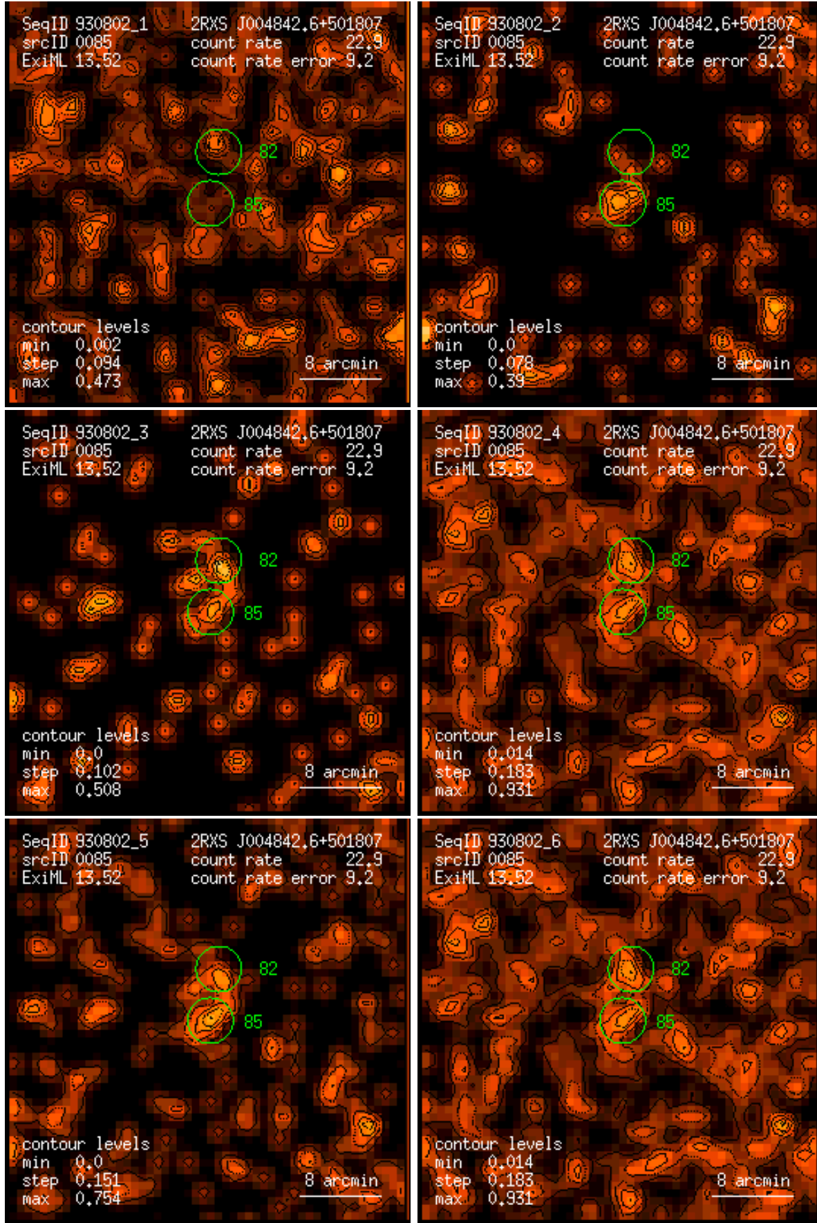
Figure 85: RASS 930802: detection 0085: band rate images, Gaussian filter: (1) PSPC channels 11 – 41, (2) 52 – 90, (3) 91 – 201, (4) 11 – 235, (5) 52 – 201, (6) 11 – 201. Broad band rates in counts/ks. Band rate contour levels in counts/ks/arcmin 2 .
