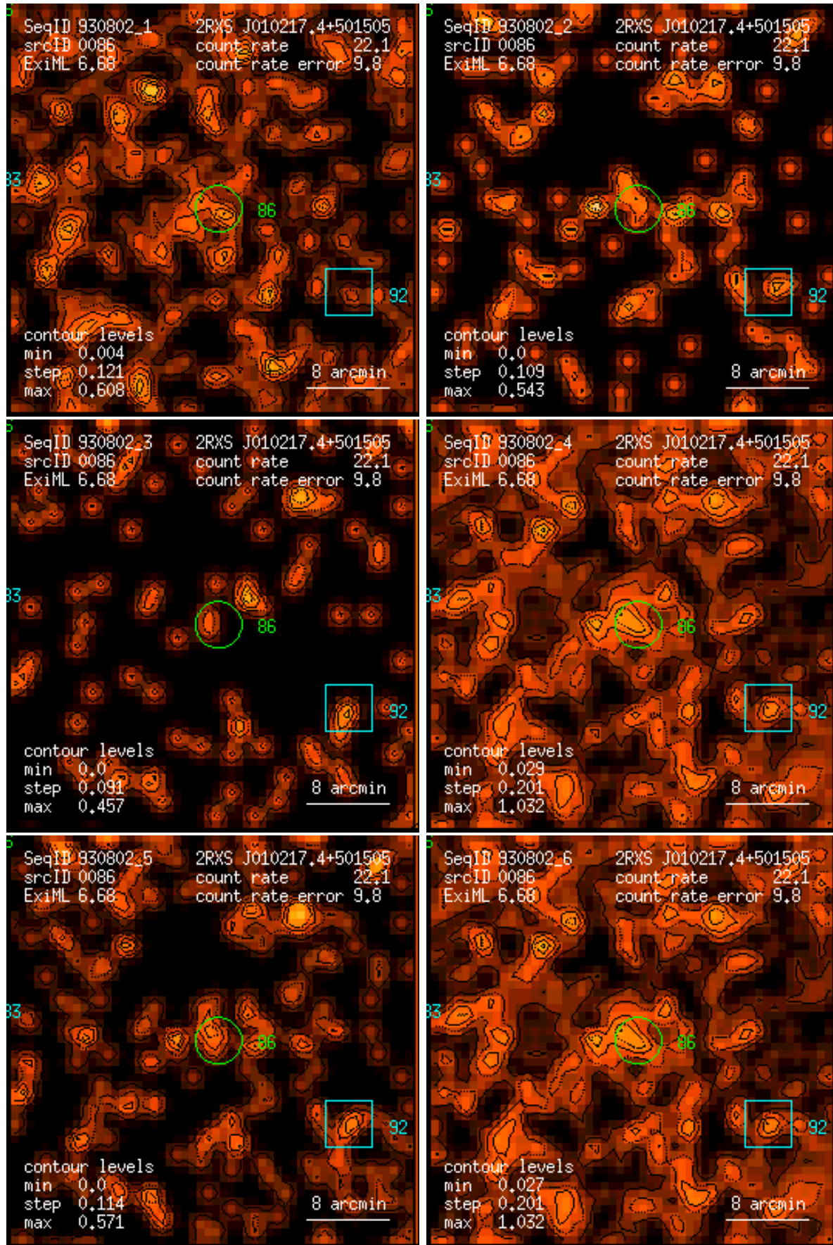
Figure 86: RASS 930802: detection 0086: band rate images, Gaussian filter: (1) PSPC channels 11 – 41, (2) 52 – 90, (3) 91 – 201, (4) 11 – 235, (5) 52 – 201, (6) 11 – 201. Broad band rates in counts/ks. Band rate contour levels in counts/ks/arcmin 2 .
