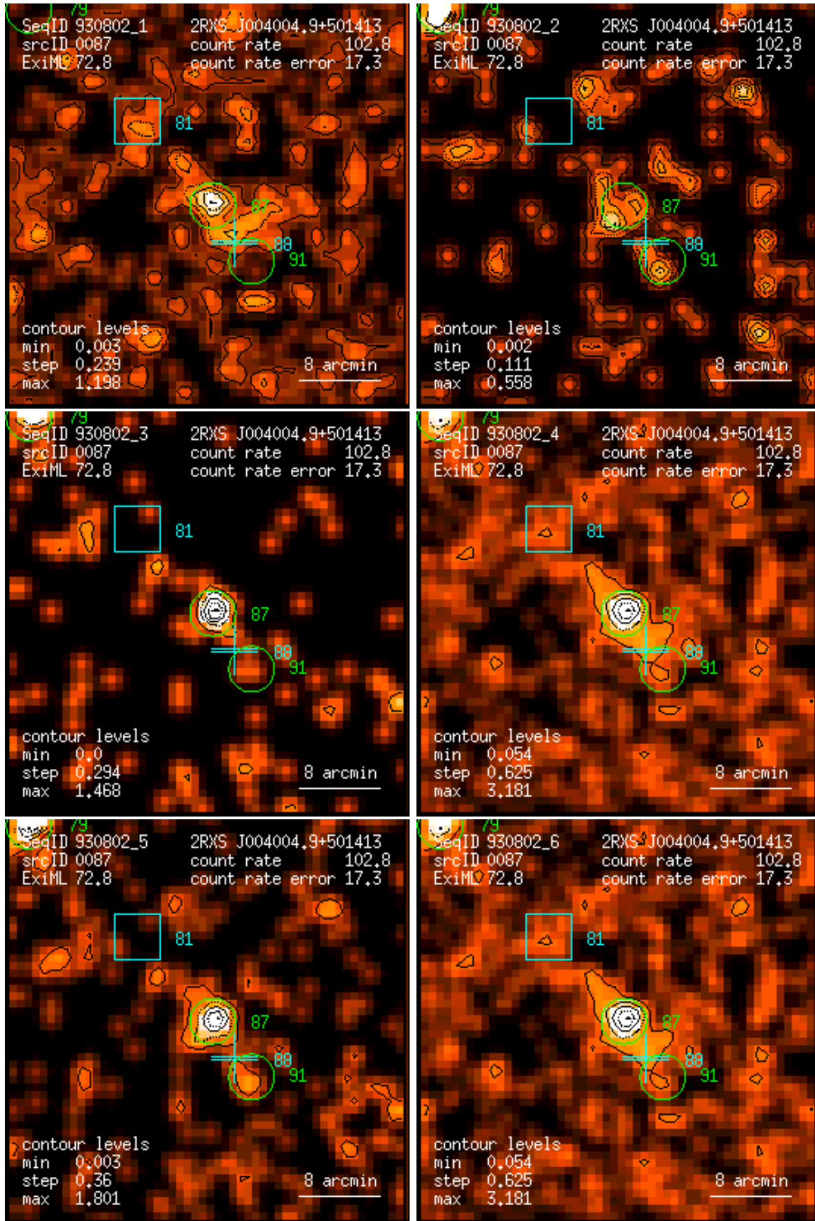
Figure 87: RASS 930802: detection 0087: band rate images, Gaussian filter: (1) PSPC channels 11 – 41, (2) 52 – 90, (3) 91 – 201, (4) 11 – 235, (5) 52 – 201, (6) 11 – 201. Broad band rates in counts/ks. Band rate contour levels in counts/ks/arcmin 2 .
