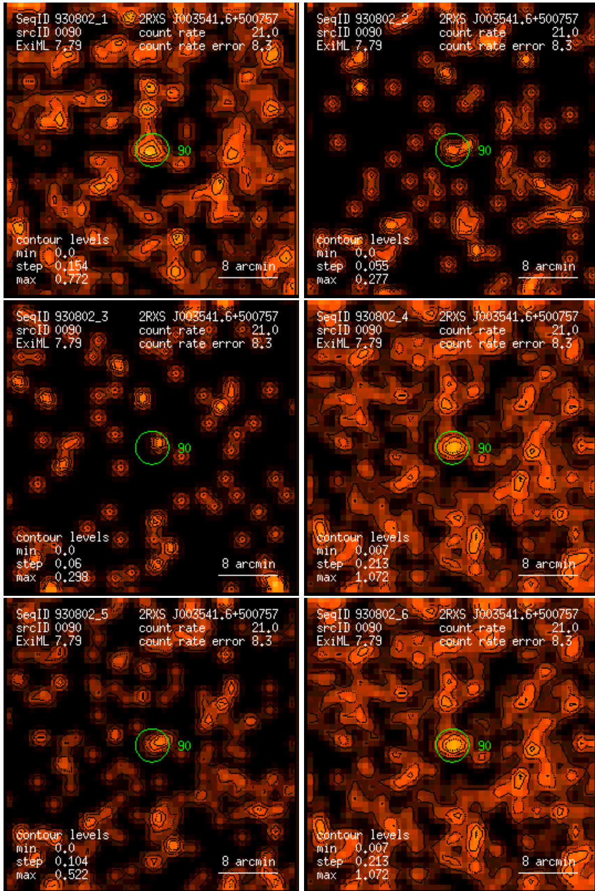
Figure 90: RASS 930802: detection 0090: band rate images, Gaussian filter: (1) PSPC channels 11 – 41, (2) 52 – 90, (3) 91 – 201, (4) 11 – 235, (5) 52 – 201, (6) 11 – 201. Broad band rates in counts/ks. Band rate contour levels in counts/ks/arcmin 2 .
