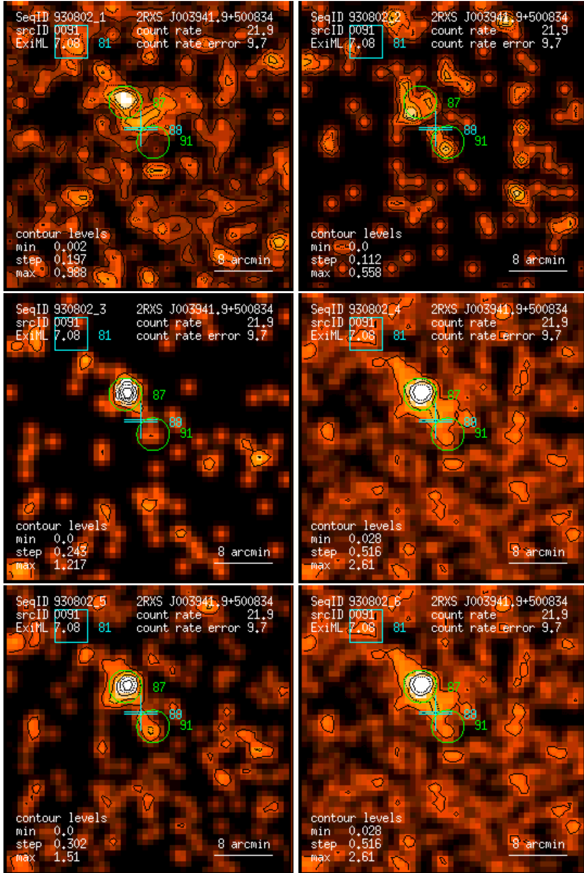
Figure 91: RASS 930802: detection 0091: band rate images, Gaussian filter: (1) PSPC channels 11 – 41, (2) 52 – 90, (3) 91 – 201, (4) 11 – 235, (5) 52 – 201, (6) 11 – 201. Broad band rates in counts/ks. Band rate contour levels in counts/ks/arcmin 2 .
