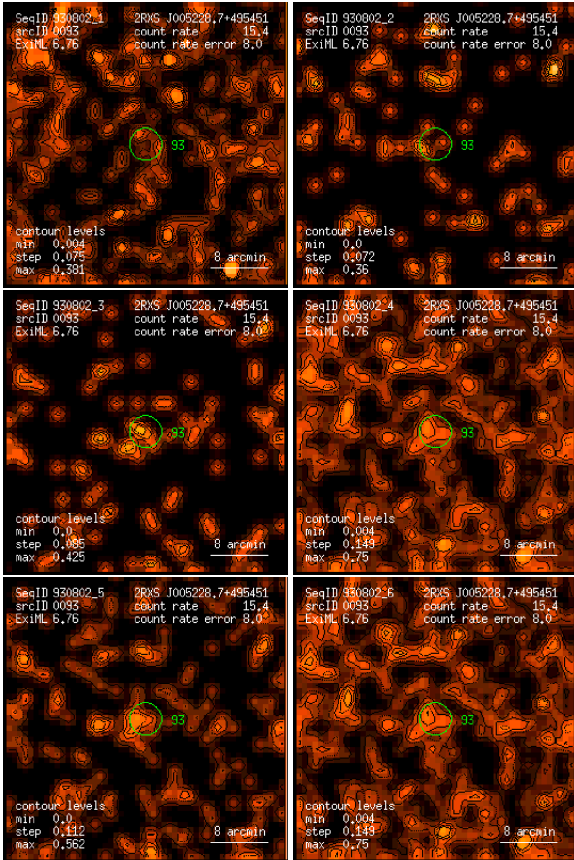
Figure 93: RASS 930802: detection 0093: band rate images, Gaussian filter: (1) PSPC channels 11 – 41, (2) 52 – 90, (3) 91 – 201, (4) 11 – 235, (5) 52 – 201, (6) 11 – 201. Broad band rates in counts/ks. Band rate contour levels in counts/ks/arcmin 2 .
