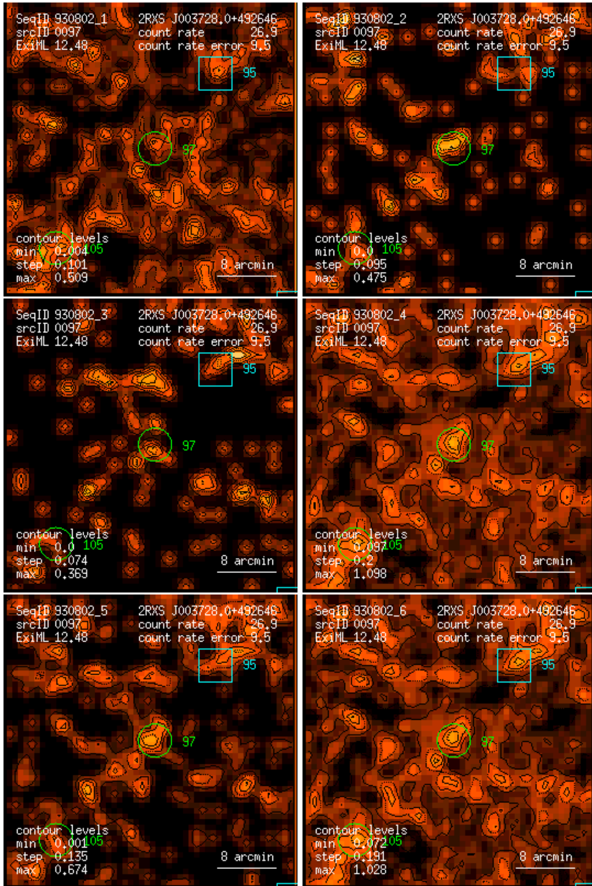
Figure 97: RASS 930802: detection 0097: band rate images, Gaussian filter: (1) PSPC channels 11 – 41, (2) 52 – 90, (3) 91 – 201, (4) 11 – 235, (5) 52 – 201, (6) 11 – 201. Broad band rates in counts/ks. Band rate contour levels in counts/ks/arcmin 2 .
