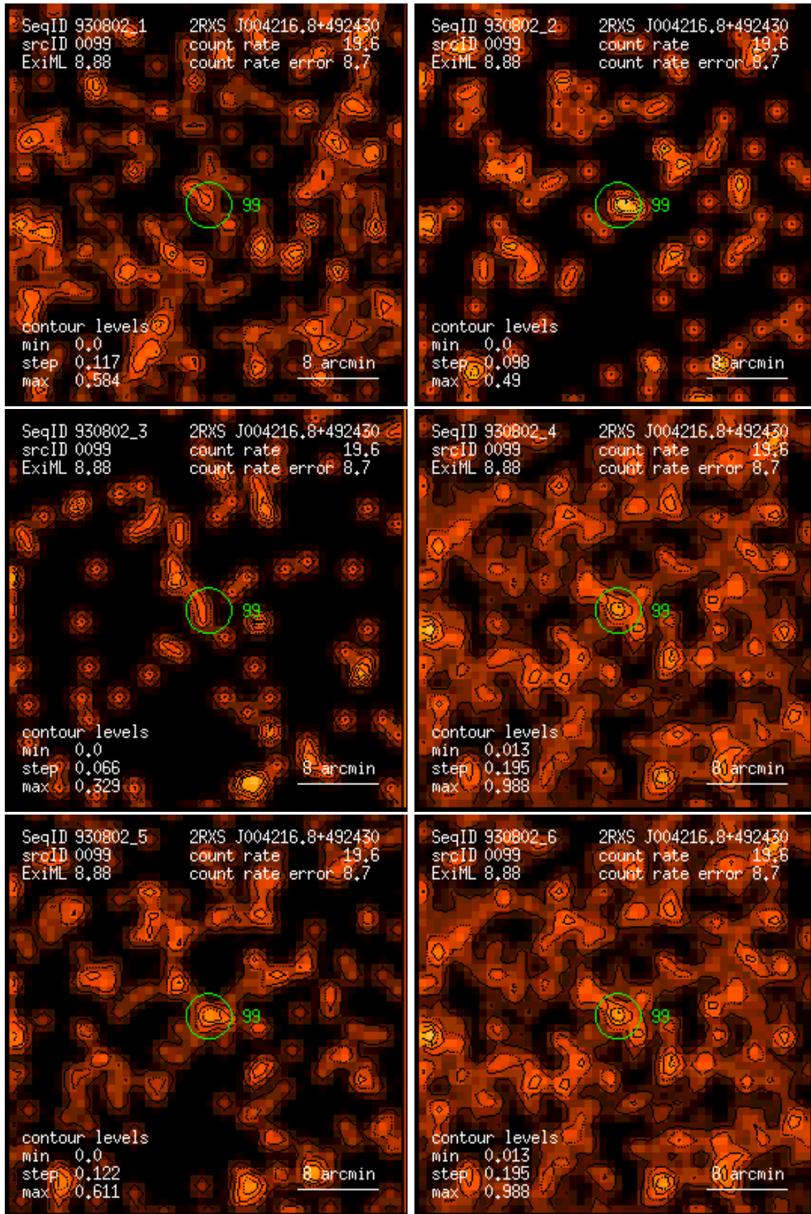
Figure 99: RASS 930802: detection 0099: band rate images, Gaussian filter: (1) PSPC channels 11 – 41, (2) 52 – 90, (3) 91 – 201, (4) 11 – 235, (5) 52 – 201, (6) 11 – 201. Broad band rates in counts/ks. Band rate contour levels in counts/ks/arcmin 2 .
