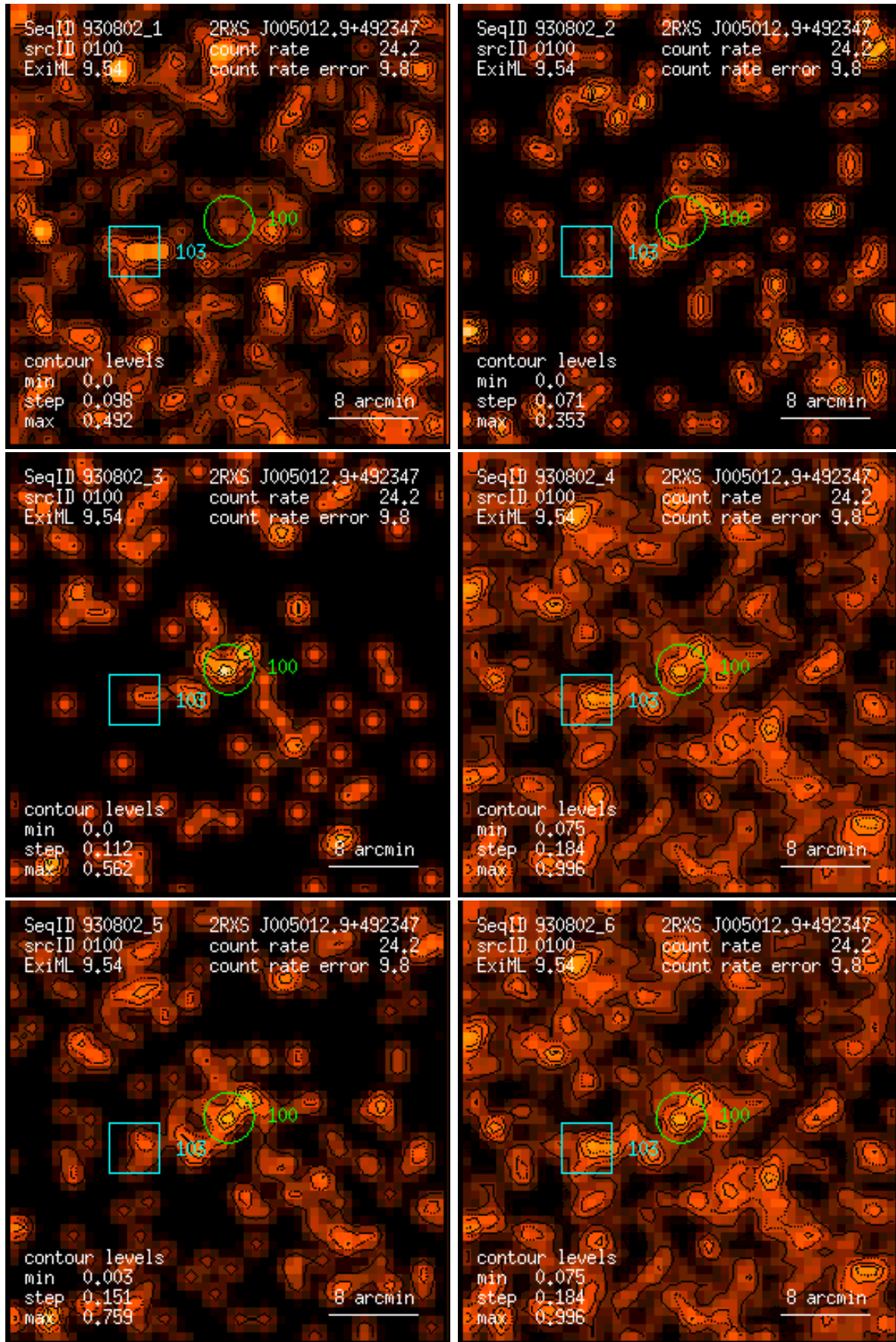
Figure 100: RASS 930802: detection 0100: band rate images, Gaussian filter: (1) PSPC channels 11 – 41, (2) 52 – 90, (3) 91 – 201, (4) 11 – 235, (5) 52 – 201, (6) 11 – 201. Broad band rates in counts/ks. Band rate contour levels in counts/ks/arcmin 2 .
