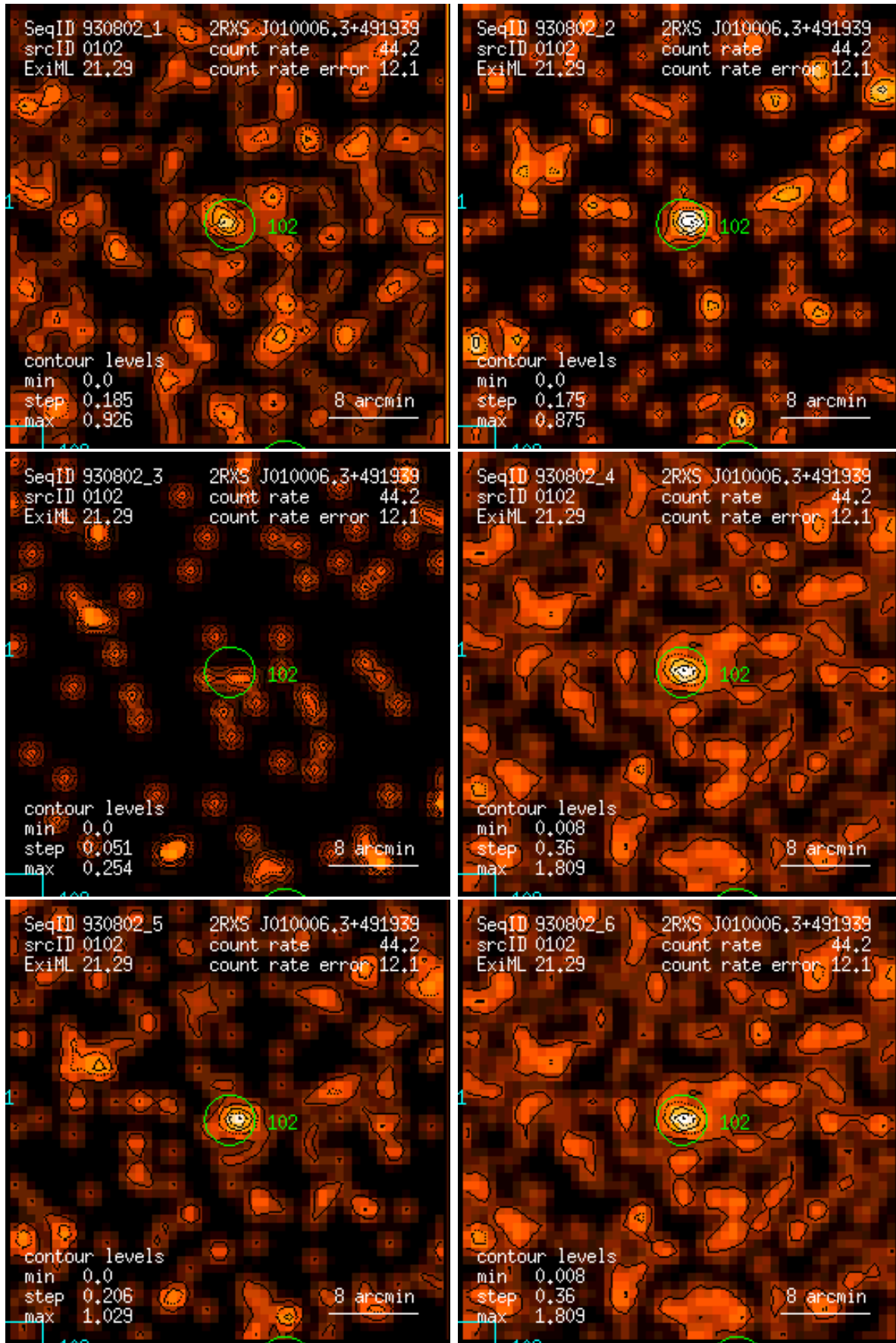
Figure 102: RASS 930802: detection 0102: band rate images, Gaussian filter: (1) PSPC channels 11 – 41, (2) 52 – 90, (3) 91 – 201, (4) 11 – 235, (5) 52 – 201, (6) 11 – 201. Broad band rates in counts/ks. Band rate contour levels in counts/ks/arcmin 2 .
