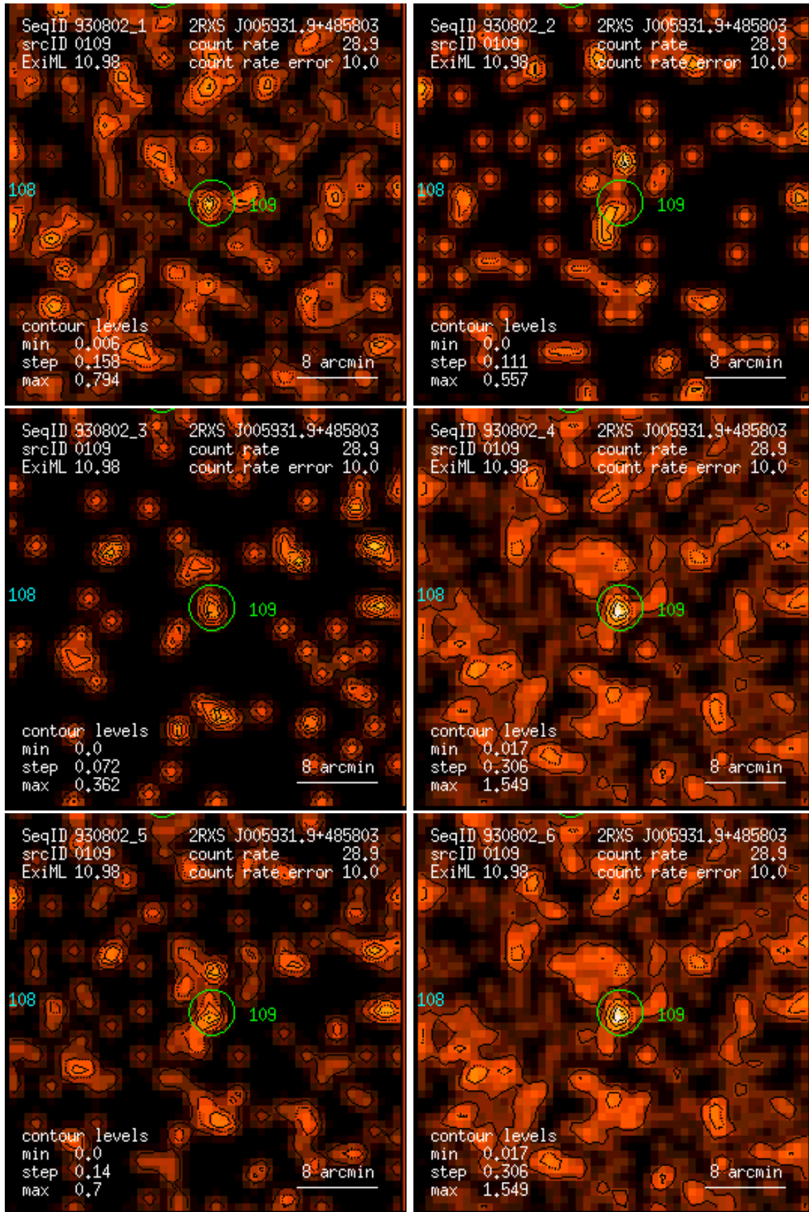
Figure 109: RASS 930802: detection 0109: band rate images, Gaussian filter: (1) PSPC channels 11 – 41, (2) 52 – 90, (3) 91 – 201, (4) 11 – 235, (5) 52 – 201, (6) 11 – 201. Broad band rates in counts/ks. Band rate contour levels in counts/ks/arcmin 2 .
