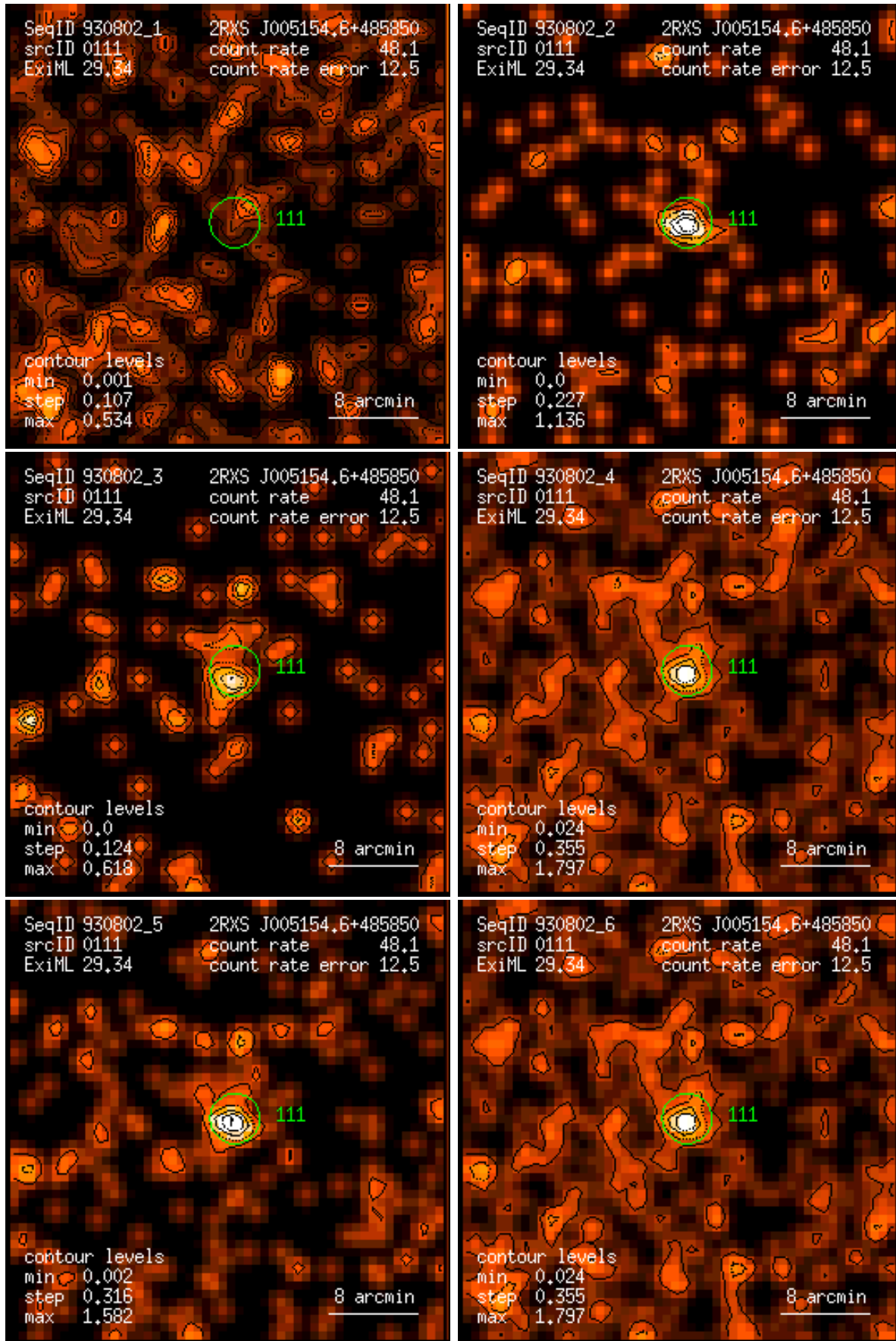
Figure 111: RASS 930802: detection 0111: band rate images, Gaussian filter: (1) PSPC channels 11 – 41, (2) 52 – 90, (3) 91 – 201, (4) 11 – 235, (5) 52 – 201, (6) 11 – 201. Broad band rates in counts/ks. Band rate contour levels in counts/ks/arcmin 2 .
