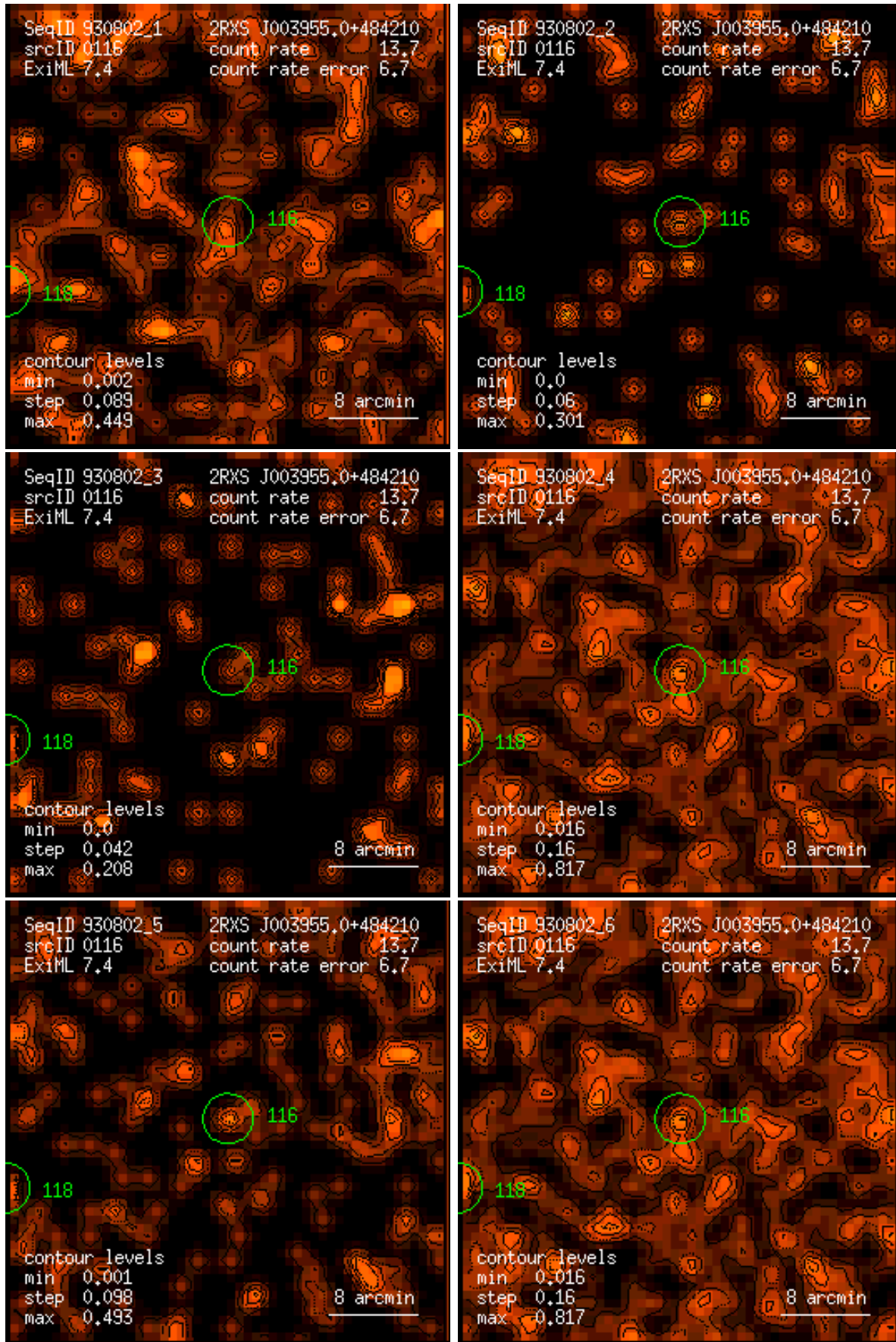
Figure 116: RASS 930802: detection 0116: band rate images, Gaussian filter: (1) PSPC channels 11 – 41, (2) 52 – 90, (3) 91 – 201, (4) 11 – 235, (5) 52 – 201, (6) 11 – 201. Broad band rates in counts/ks. Band rate contour levels in counts/ks/arcmin 2 .
