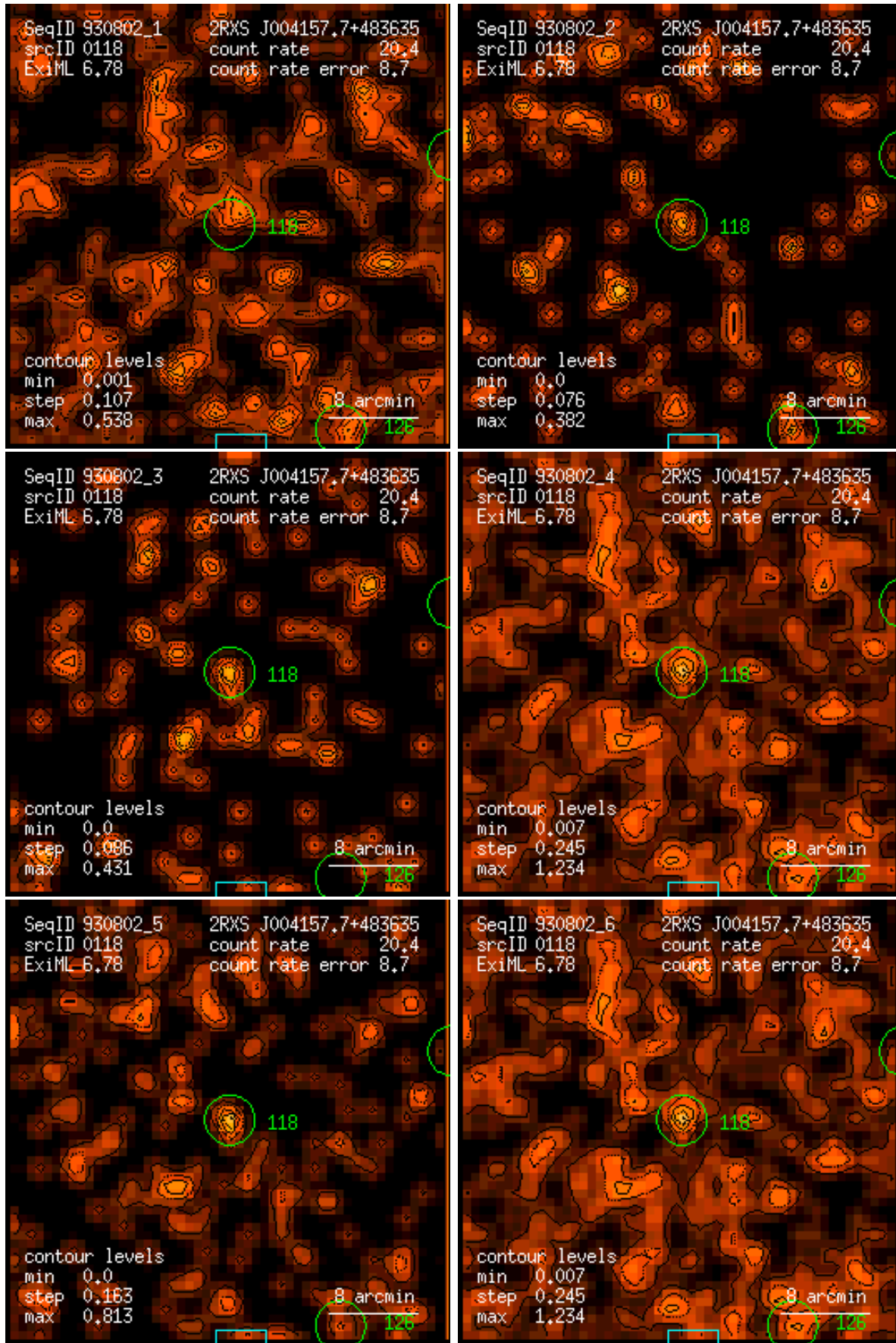
Figure 118: RASS 930802: detection 0118: band rate images, Gaussian filter: (1) PSPC channels 11 – 41, (2) 52 – 90, (3) 91 – 201, (4) 11 – 235, (5) 52 – 201, (6) 11 – 201. Broad band rates in counts/ks. Band rate contour levels in counts/ks/arcmin 2 .
