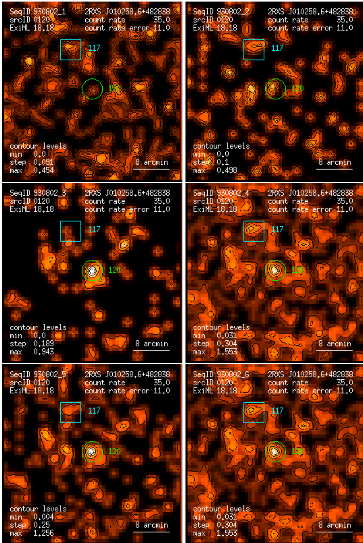
Figure 120: RASS 930802: detection 0120: band rate images, Gaussian filter: (1) PSPC channels 11 – 41, (2) 52 – 90, (3) 91 – 201, (4) 11 – 235, (5) 52 – 201, (6) 11 – 201. Broad band rates in counts/ks. Band rate contour levels in counts/ks/arcmin 2 .
