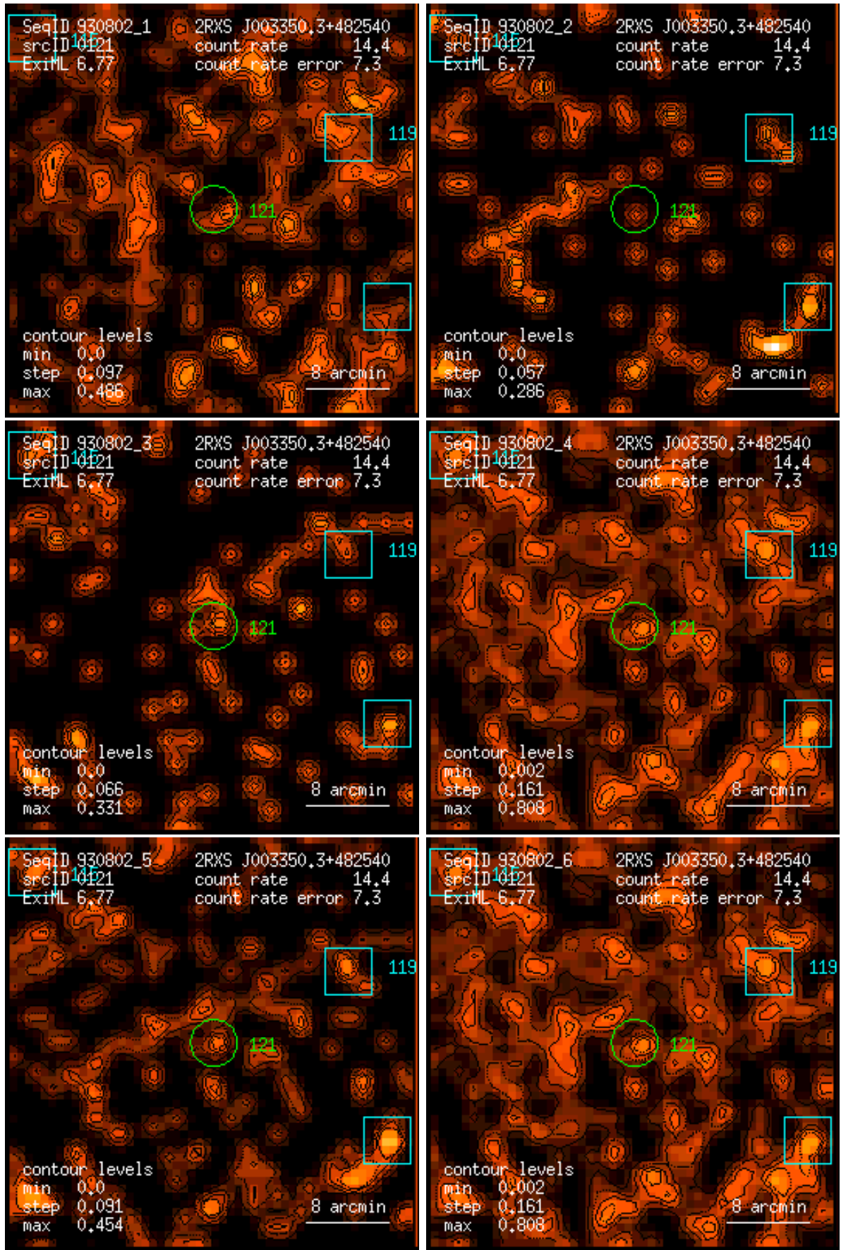
Figure 121: RASS 930802: detection 0121: band rate images, Gaussian filter: (1) PSPC channels 11 – 41, (2) 52 – 90, (3) 91 – 201, (4) 11 – 235, (5) 52 – 201, (6) 11 – 201. Broad band rates in counts/ks. Band rate contour levels in counts/ks/arcmin 2 .
