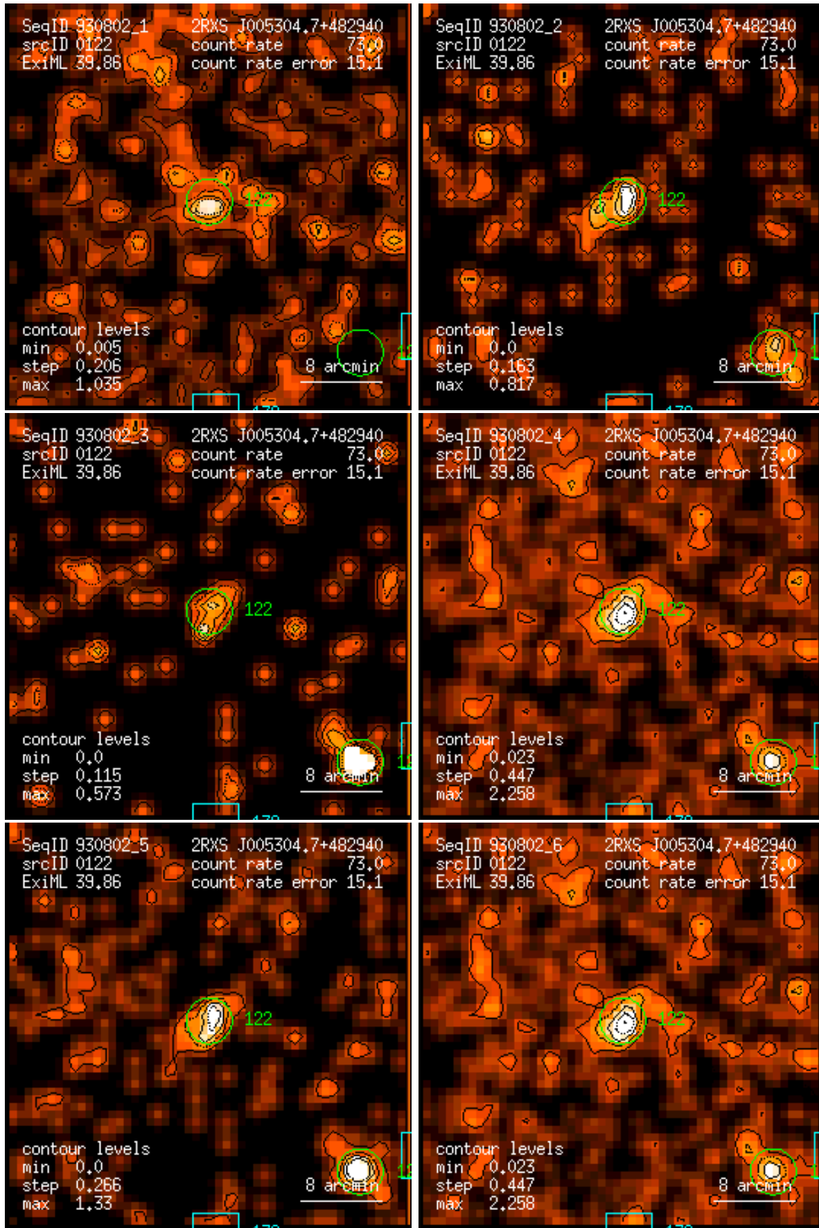
Figure 122: RASS 930802: detection 0122: band rate images, Gaussian filter: (1) PSPC channels 11 – 41, (2) 52 – 90, (3) 91 – 201, (4) 11 – 235, (5) 52 – 201, (6) 11 – 201. Broad band rates in counts/ks. Band rate contour levels in counts/ks/arcmin 2 .
