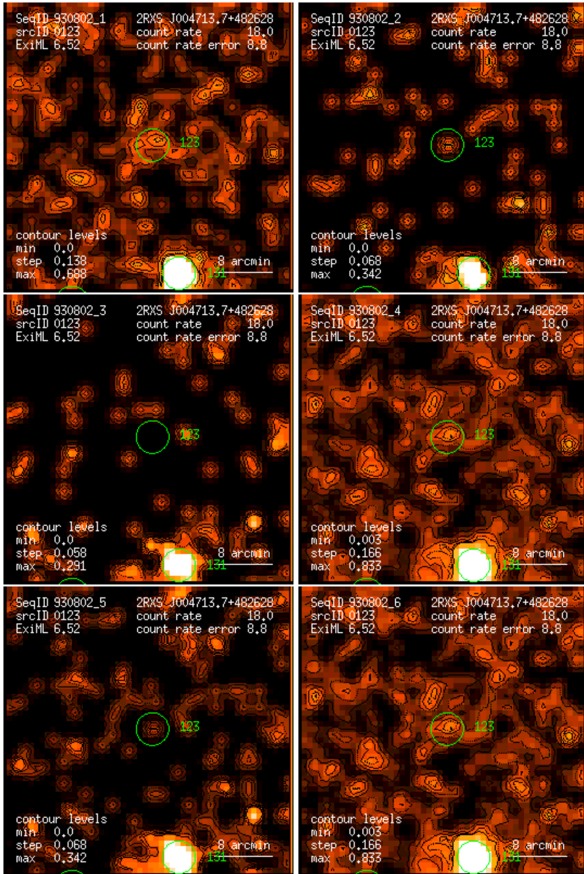
Figure 123: RASS 930802: detection 0123: band rate images, Gaussian filter: (1) PSPC channels 11 – 41, (2) 52 – 90, (3) 91 – 201, (4) 11 – 235, (5) 52 – 201, (6) 11 – 201. Broad band rates in counts/ks. Band rate contour levels in counts/ks/arcmin 2 .
