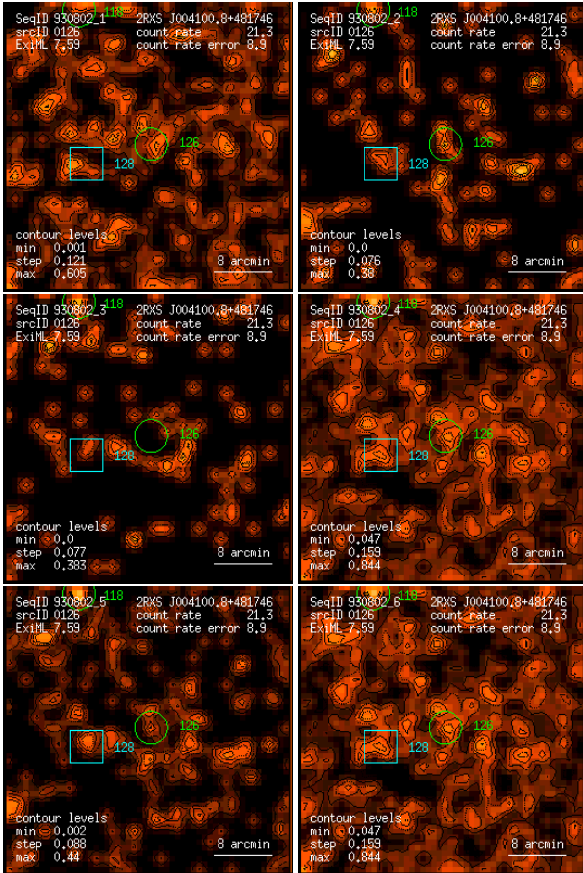
Figure 126: RASS 930802: detection 0126: band rate images, Gaussian filter: (1) PSPC channels 11 – 41, (2) 52 – 90, (3) 91 – 201, (4) 11 – 235, (5) 52 – 201, (6) 11 – 201. Broad band rates in counts/ks. Band rate contour levels in counts/ks/arcmin 2 .
