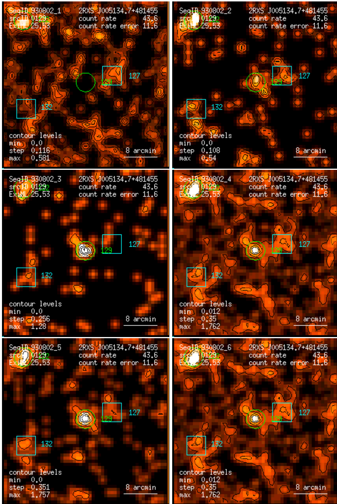
Figure 129: RASS 930802: detection 0129: band rate images, Gaussian filter: (1) PSPC channels 11 – 41, (2) 52 – 90, (3) 91 – 201, (4) 11 – 235, (5) 52 – 201, (6) 11 – 201. Broad band rates in counts/ks. Band rate contour levels in counts/ks/arcmin 2 .
