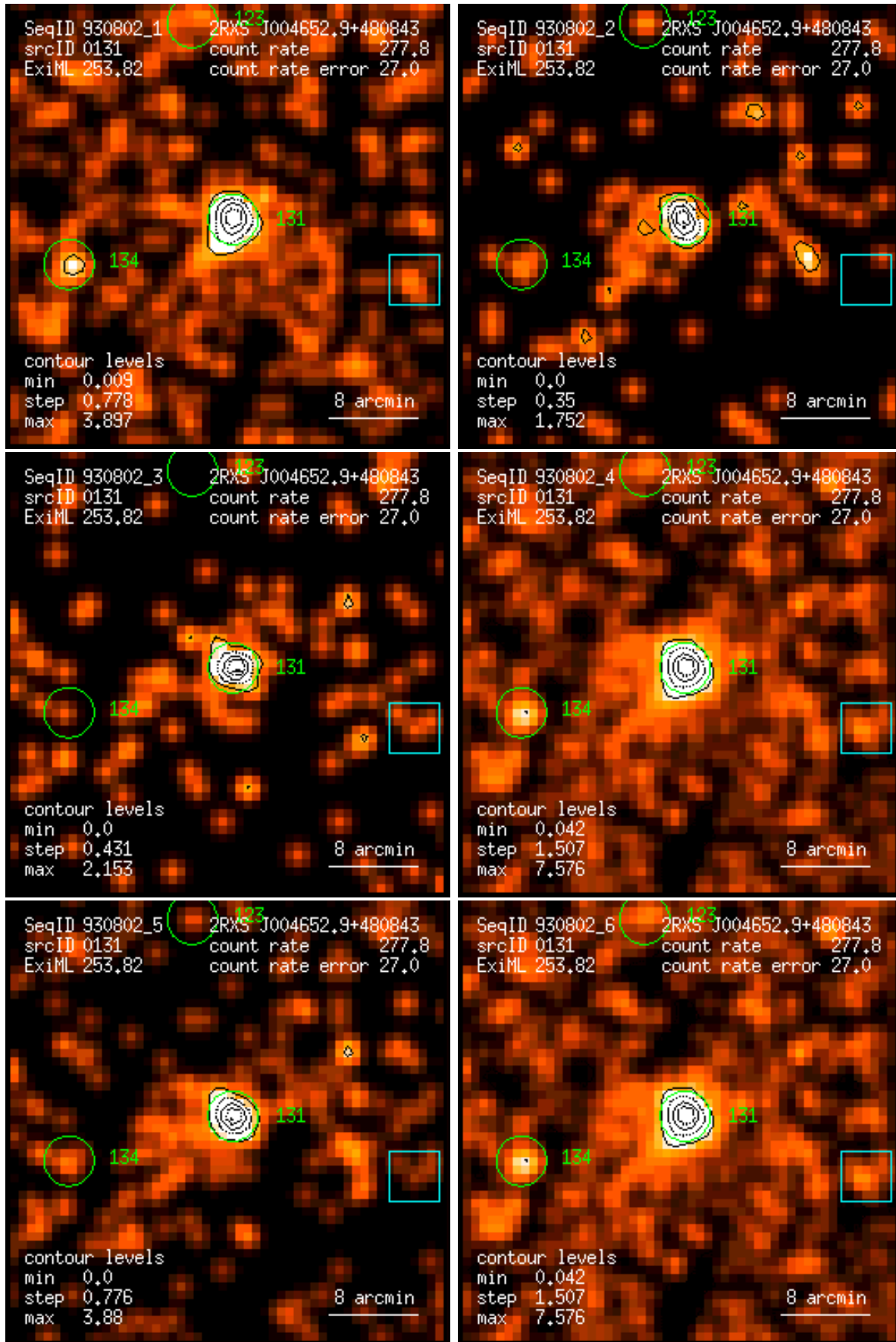
Figure 131: RASS 930802: detection 0131: band rate images, Gaussian filter: (1) PSPC channels 11 – 41, (2) 52 – 90, (3) 91 – 201, (4) 11 – 235, (5) 52 – 201, (6) 11 – 201. Broad band rates in counts/ks. Band rate contour levels in counts/ks/arcmin 2 .
