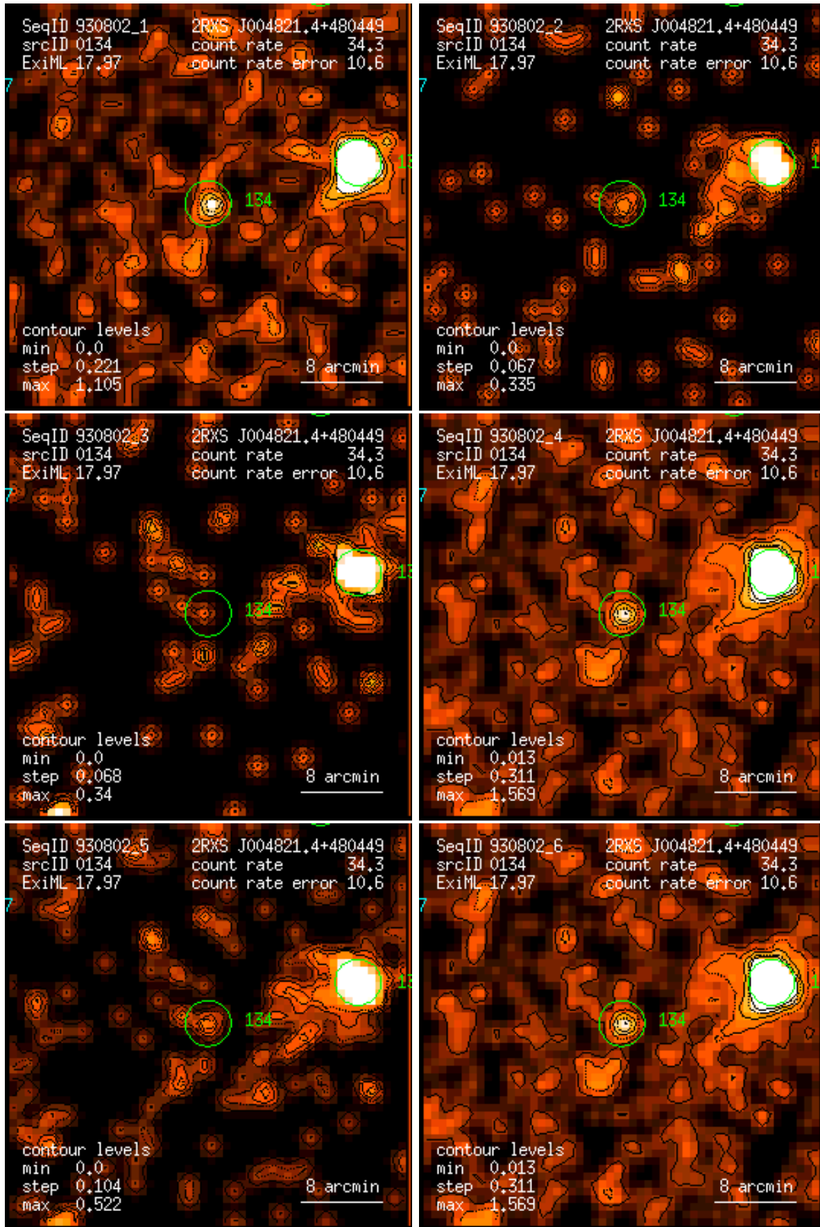
Figure 134: RASS 930802: detection 0134: band rate images, Gaussian filter: (1) PSPC channels 11 – 41, (2) 52 – 90, (3) 91 – 201, (4) 11 – 235, (5) 52 – 201, (6) 11 – 201. Broad band rates in counts/ks. Band rate contour levels in counts/ks/arcmin 2 .
