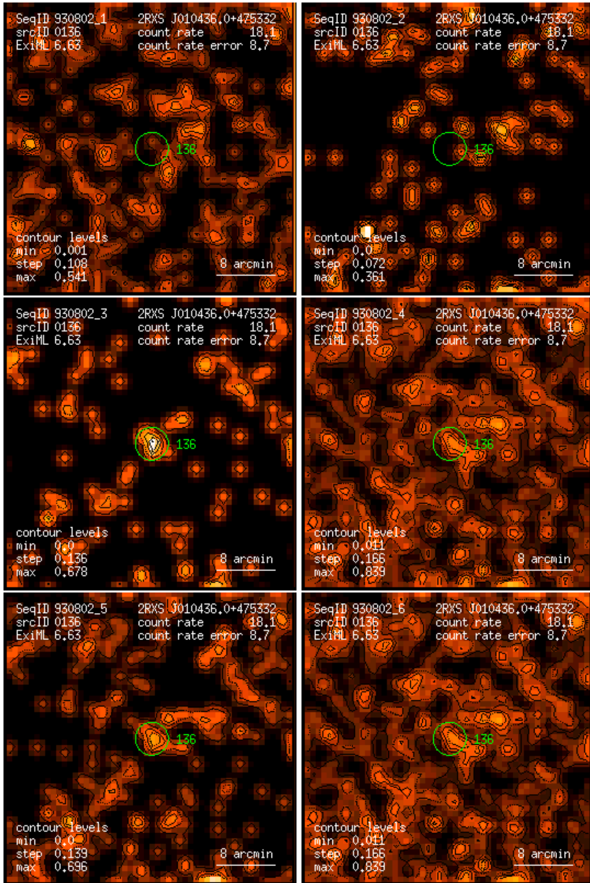
Figure 136: RASS 930802: detection 0136: band rate images, Gaussian filter: (1) PSPC channels 11 – 41, (2) 52 – 90, (3) 91 – 201, (4) 11 – 235, (5) 52 – 201, (6) 11 – 201. Broad band rates in counts/ks. Band rate contour levels in counts/ks/arcmin 2 .
