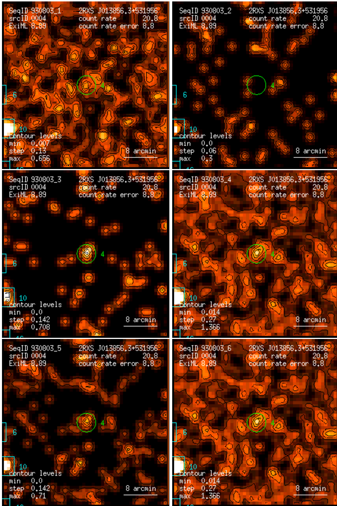
Figure 4: RASS 930803: detection 0004: band rate images, Gaussian filter: (1) PSPC channels 11 – 41, (2) 52 – 90, (3) 91 – 201, (4) 11 – 235, (5) 52 – 201, (6) 11 – 201. Broad band rates in counts/ks. Band rate contour levels in counts/ks/arcmin 2 .
