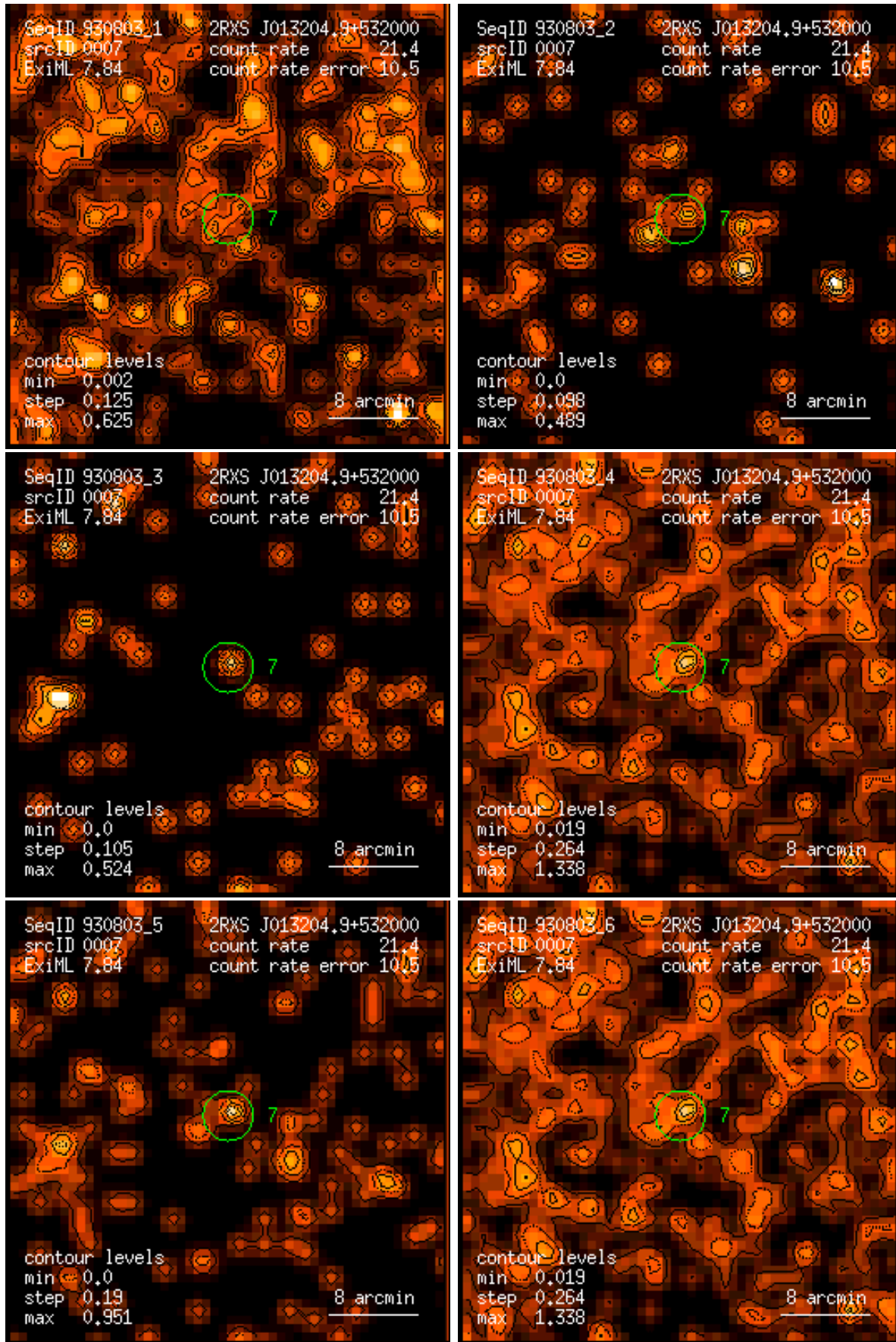
Figure 7: RASS 930803: detection 0007: band rate images, Gaussian filter: (1) PSPC channels 11 – 41, (2) 52 – 90, (3) 91 – 201, (4) 11 – 235, (5) 52 – 201, (6) 11 – 201. Broad band rates in counts/ks. Band rate contour levels in counts/ks/arcmin 2 .
