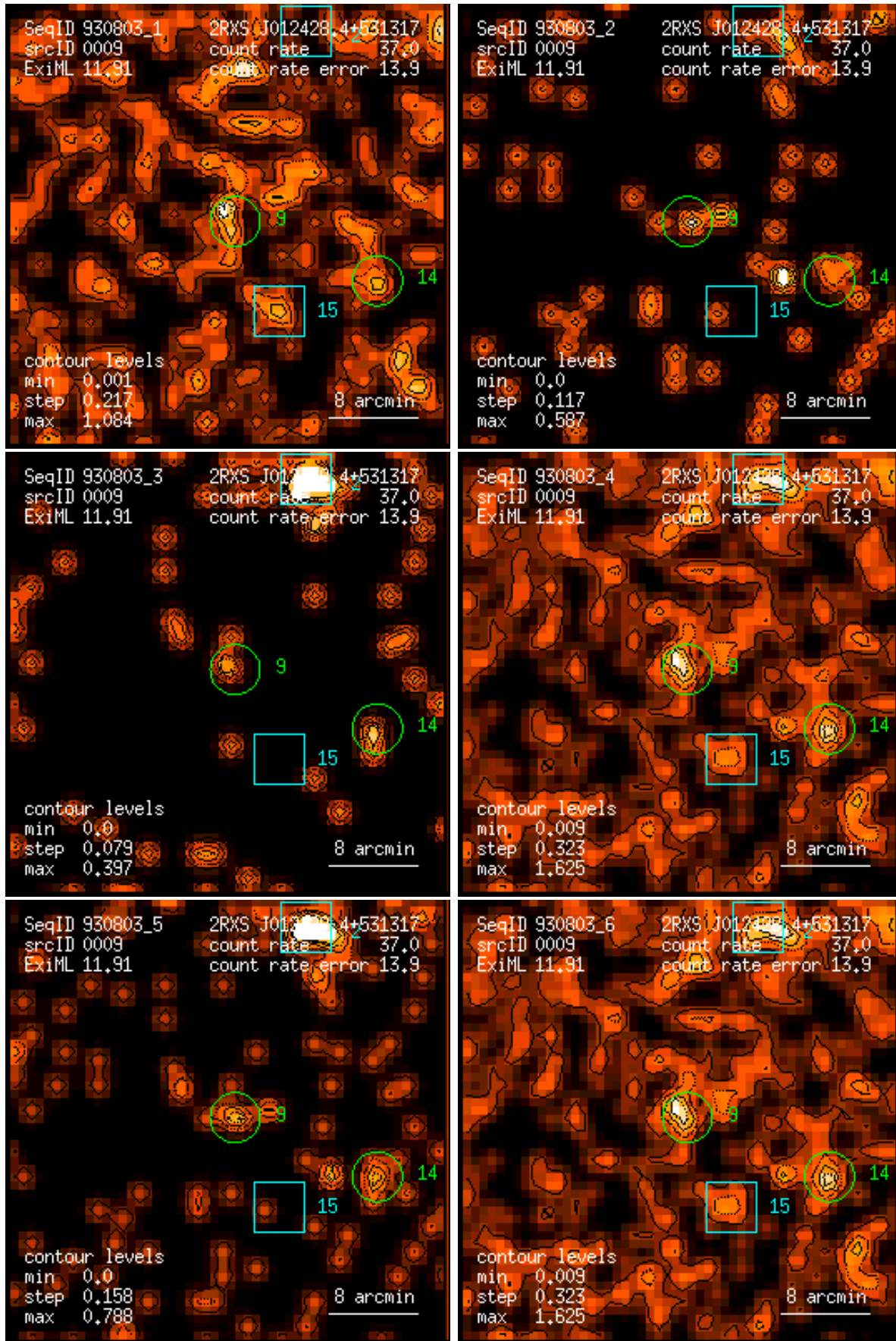
Figure 9: RASS 930803: detection 0009: band rate images, Gaussian filter: (1) PSPC channels 11 – 41, (2) 52 – 90, (3) 91 – 201, (4) 11 – 235, (5) 52 – 201, (6) 11 – 201. Broad band rates in counts/ks. Band rate contour levels in counts/ks/arcmin 2 .
