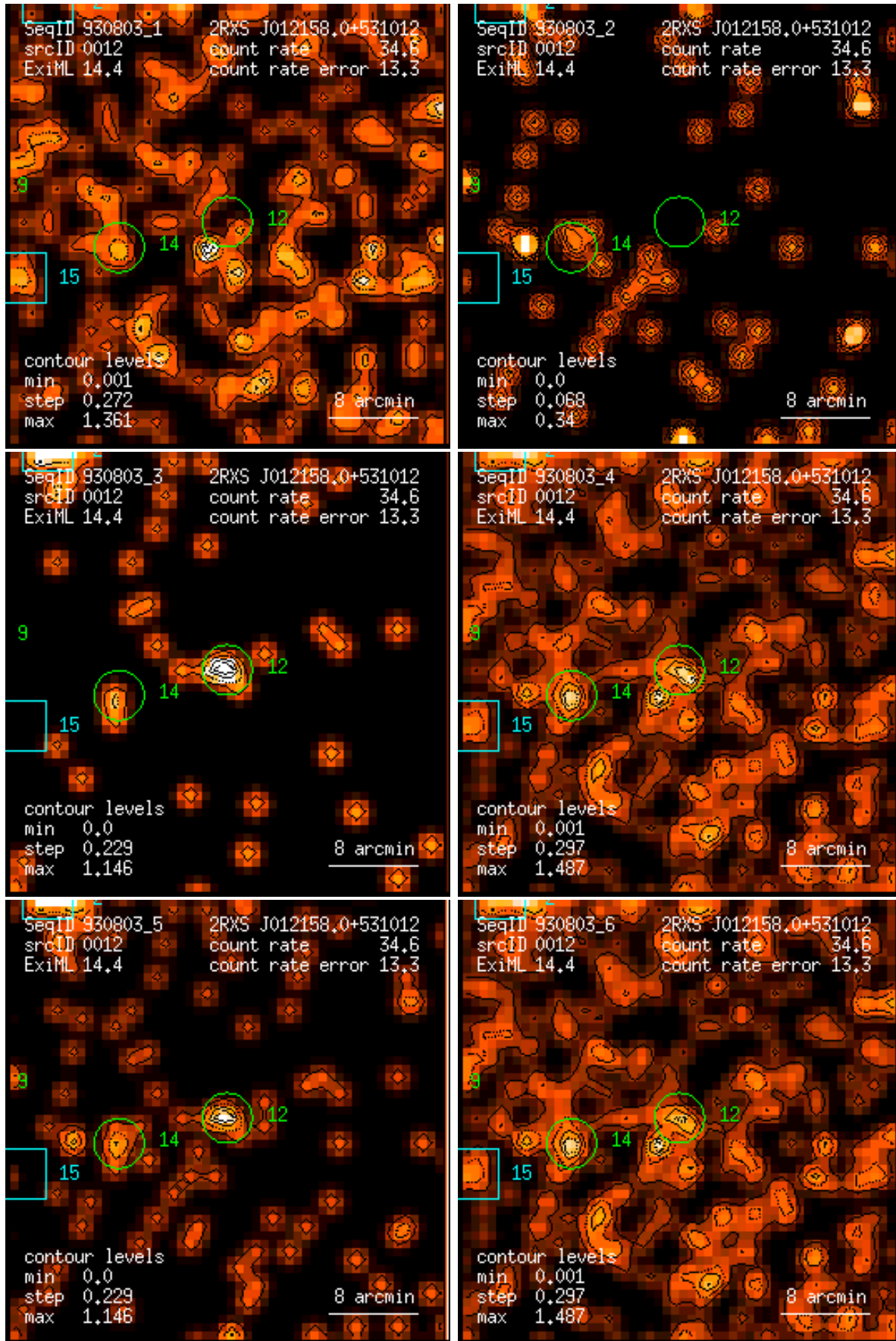
Figure 12: RASS 930803: detection 0012: band rate images, Gaussian filter: (1) PSPC channels 11 – 41, (2) 52 – 90, (3) 91 – 201, (4) 11 – 235, (5) 52 – 201, (6) 11 – 201. Broad band rates in counts/ks. Band rate contour levels in counts/ks/arcmin 2 .
