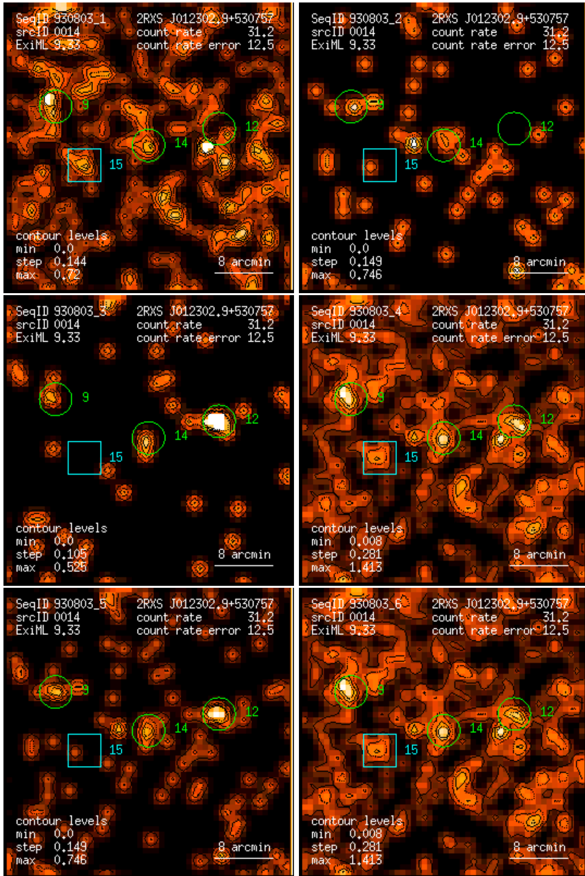
Figure 14: RASS 930803: detection 0014: band rate images, Gaussian filter: (1) PSPC channels 11 – 41, (2) 52 – 90, (3) 91 – 201, (4) 11 – 235, (5) 52 – 201, (6) 11 – 201. Broad band rates in counts/ks. Band rate contour levels in counts/ks/arcmin 2 .
