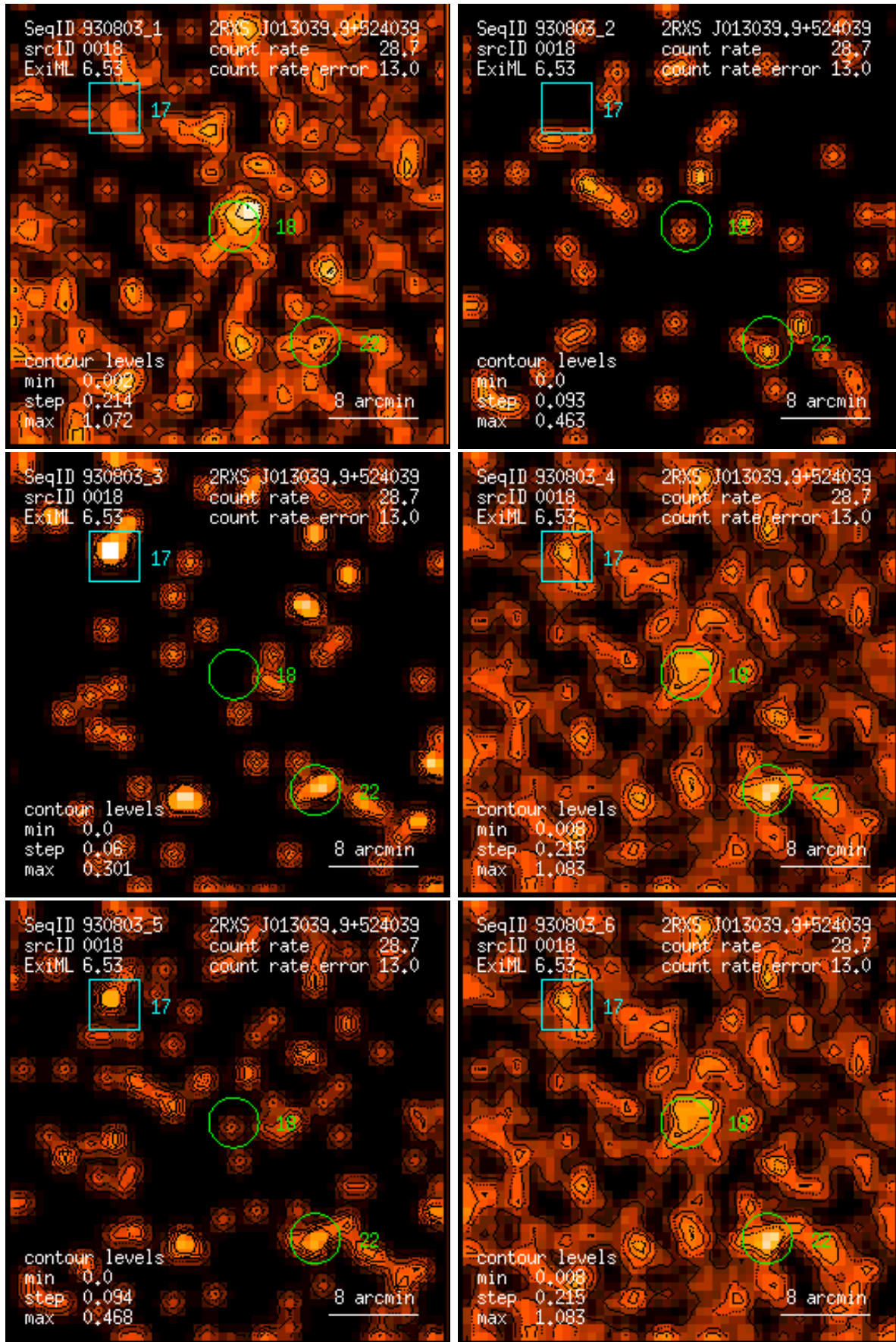
Figure 18: RASS 930803: detection 0018: band rate images, Gaussian filter: (1) PSPC channels 11 – 41, (2) 52 – 90, (3) 91 – 201, (4) 11 – 235, (5) 52 – 201, (6) 11 – 201. Broad band rates in counts/ks. Band rate contour levels in counts/ks/arcmin 2 .
