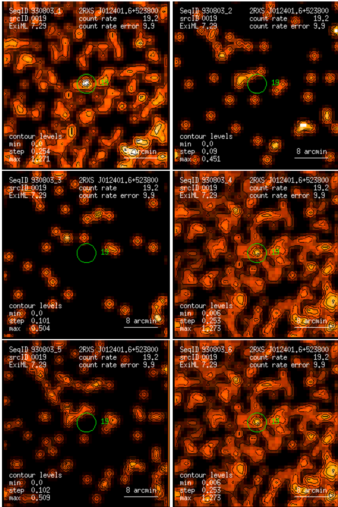
Figure 19: RASS 930803: detection 0019: band rate images, Gaussian filter: (1) PSPC channels 11 – 41, (2) 52 – 90, (3) 91 – 201, (4) 11 – 235, (5) 52 – 201, (6) 11 – 201. Broad band rates in counts/ks. Band rate contour levels in counts/ks/arcmin 2 .
