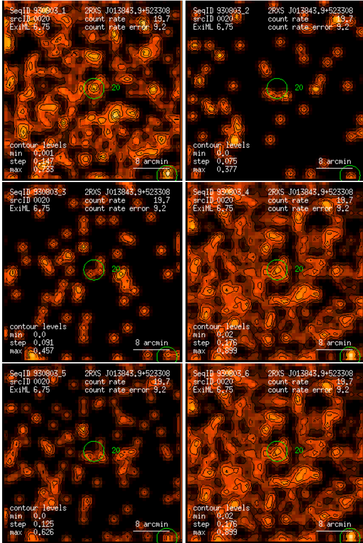
Figure 20: RASS 930803: detection 0020: band rate images, Gaussian filter: (1) PSPC channels 11 – 41, (2) 52 – 90, (3) 91 – 201, (4) 11 – 235, (5) 52 – 201, (6) 11 – 201. Broad band rates in counts/ks. Band rate contour levels in counts/ks/arcmin 2 .
