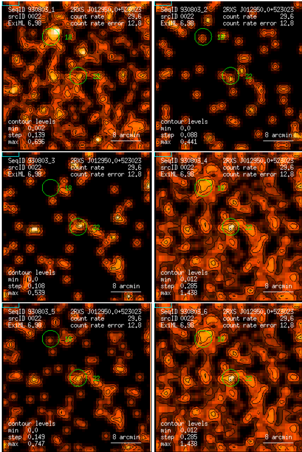
Figure 22: RASS 930803: detection 0022: band rate images, Gaussian filter: (1) PSPC channels 11 – 41, (2) 52 – 90, (3) 91 – 201, (4) 11 – 235, (5) 52 – 201, (6) 11 – 201. Broad band rates in counts/ks. Band rate contour levels in counts/ks/arcmin 2 .
