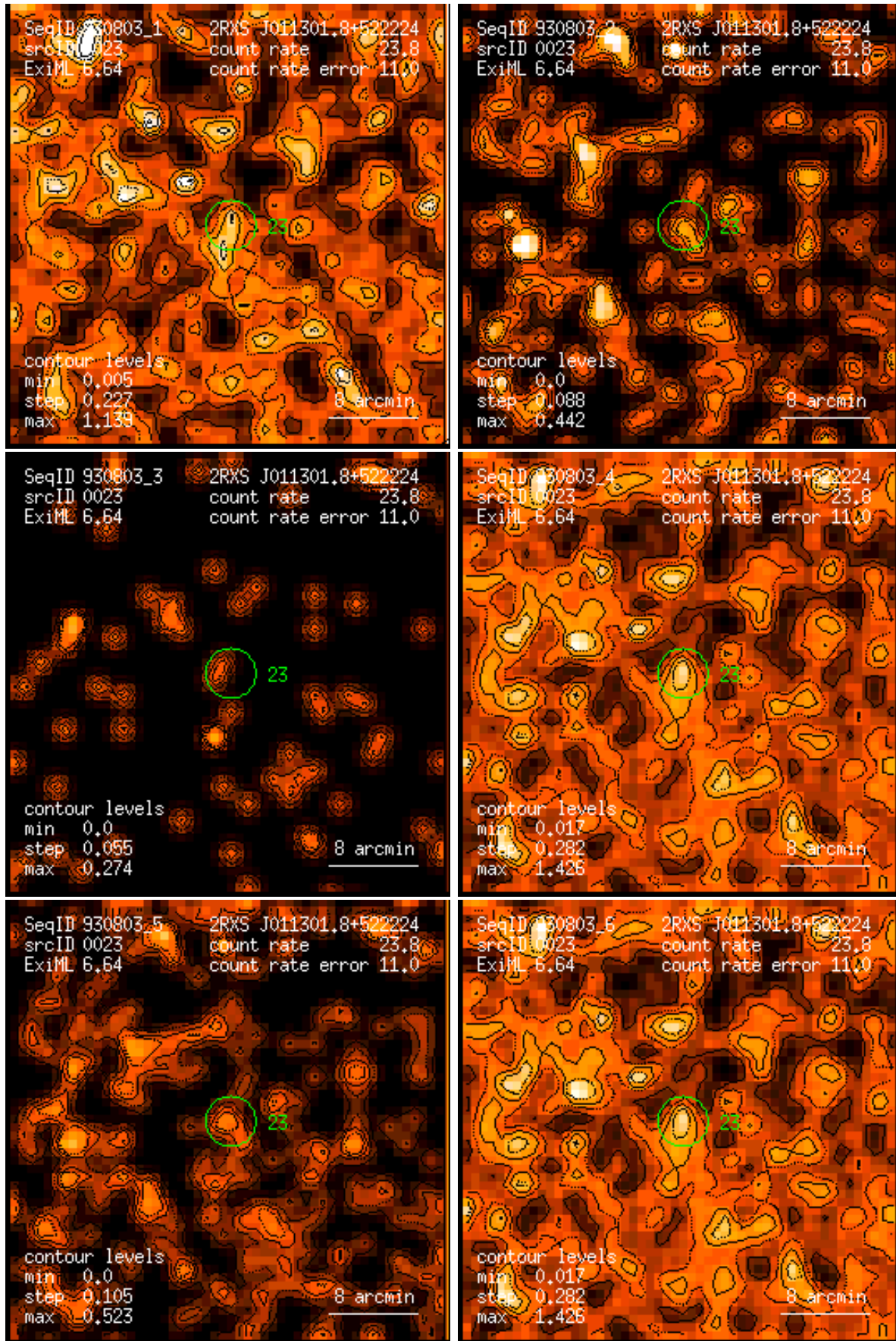
Figure 23: RASS 930803: detection 0023: band rate images, Gaussian filter: (1) PSPC channels 11 – 41, (2) 52 – 90, (3) 91 – 201, (4) 11 – 235, (5) 52 – 201, (6) 11 – 201. Broad band rates in counts/ks. Band rate contour levels in counts/ks/arcmin 2 .
