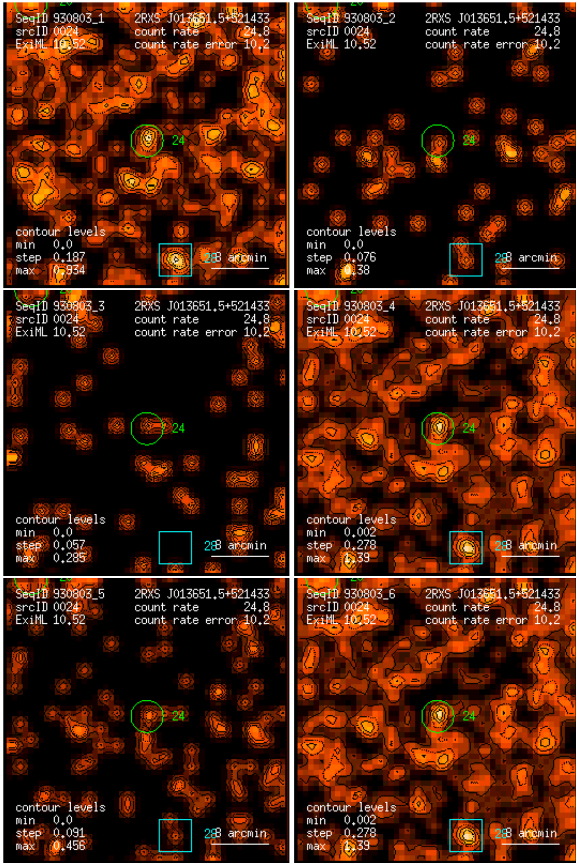
Figure 24: RASS 930803: detection 0024: band rate images, Gaussian filter: (1) PSPC channels 11 – 41, (2) 52 – 90, (3) 91 – 201, (4) 11 – 235, (5) 52 – 201, (6) 11 – 201. Broad band rates in counts/ks. Band rate contour levels in counts/ks/arcmin 2 .
