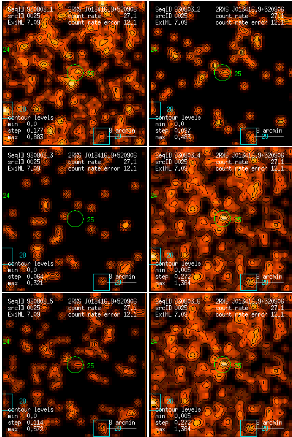
Figure 25: RASS 930803: detection 0025: band rate images, Gaussian filter: (1) PSPC channels 11 – 41, (2) 52 – 90, (3) 91 – 201, (4) 11 – 235, (5) 52 – 201, (6) 11 – 201. Broad band rates in counts/ks. Band rate contour levels in counts/ks/arcmin 2 .
