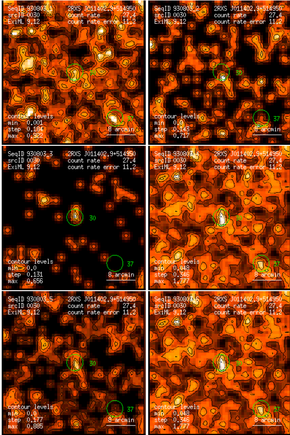
Figure 30: RASS 930803: detection 0030: band rate images, Gaussian filter: (1) PSPC channels 11 – 41, (2) 52 – 90, (3) 91 – 201, (4) 11 – 235, (5) 52 – 201, (6) 11 – 201. Broad band rates in counts/ks. Band rate contour levels in counts/ks/arcmin 2 .
